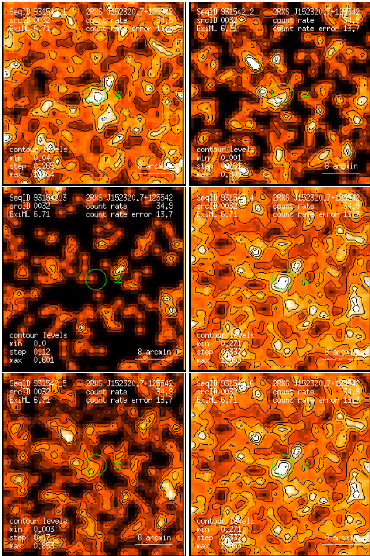
Figure 32: RASS 931542: detection 0032: band rate images, Gaussian filter: (1) PSPC channels 11 – 41, (2) 52 – 90, (3) 91 – 201, (4) 11 – 235, (5) 52 – 201, (6) 11 – 201. Broad band rates in counts/ks. Band rate contour levels in counts/ks/arcmin 2 .
