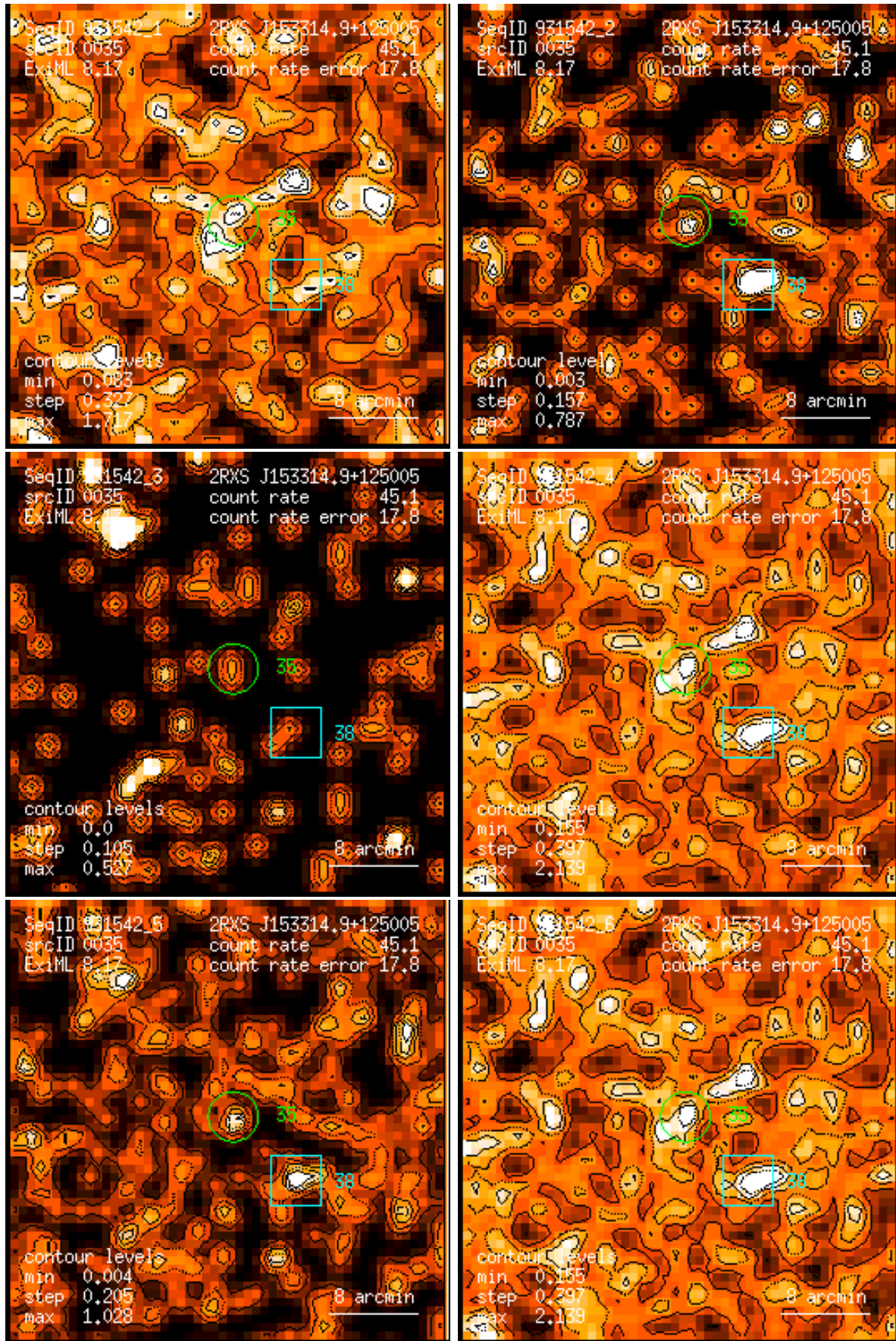
Figure 35: RASS 931542: detection 0035: band rate images, Gaussian filter: (1) PSPC channels 11 – 41, (2) 52 – 90, (3) 91 – 201, (4) 11 – 235, (5) 52 – 201, (6) 11 – 201. Broad band rates in counts/ks. Band rate contour levels in counts/ks/arcmin 2 .
