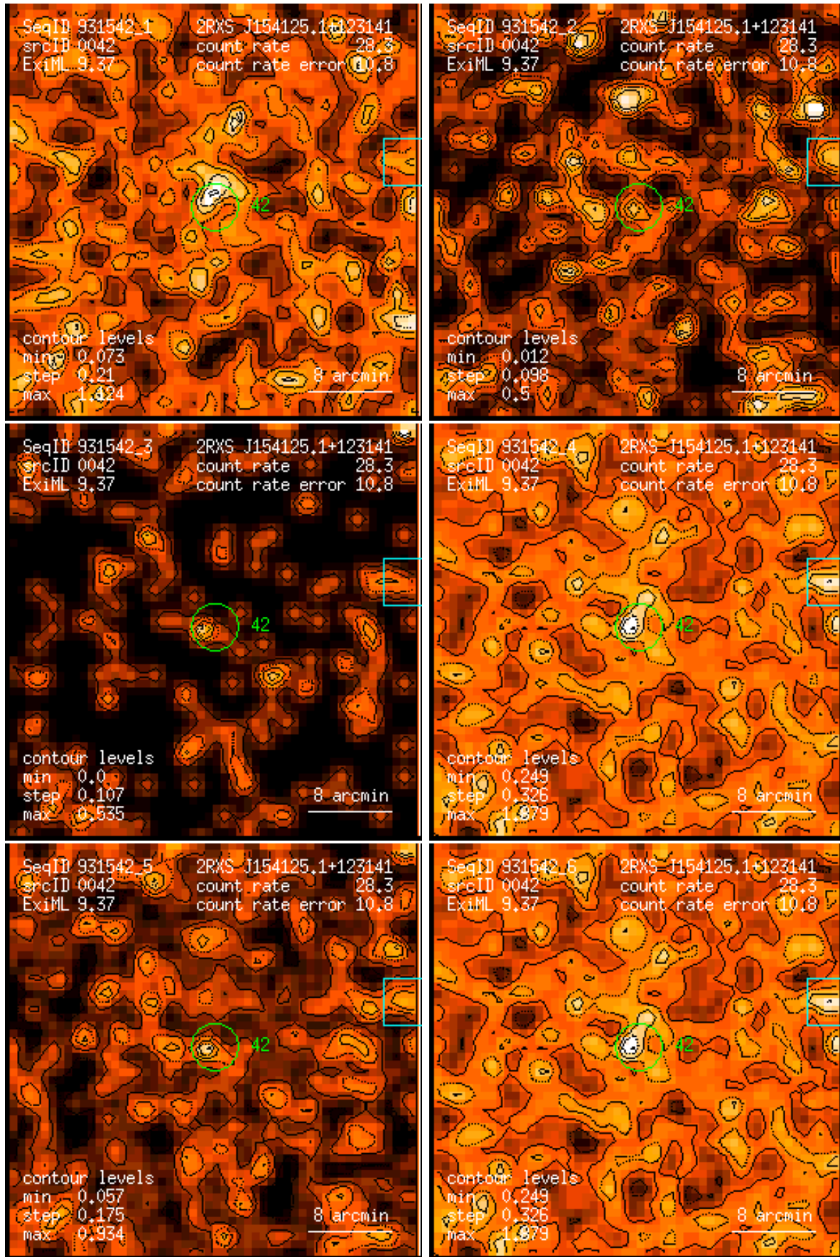
Figure 42: RASS 931542: detection 0042: band rate images, Gaussian filter: (1) PSPC channels 11 – 41, (2) 52 – 90, (3) 91 – 201, (4) 11 – 235, (5) 52 – 201, (6) 11 – 201. Broad band rates in counts/ks. Band rate contour levels in counts/ks/arcmin 2 .
