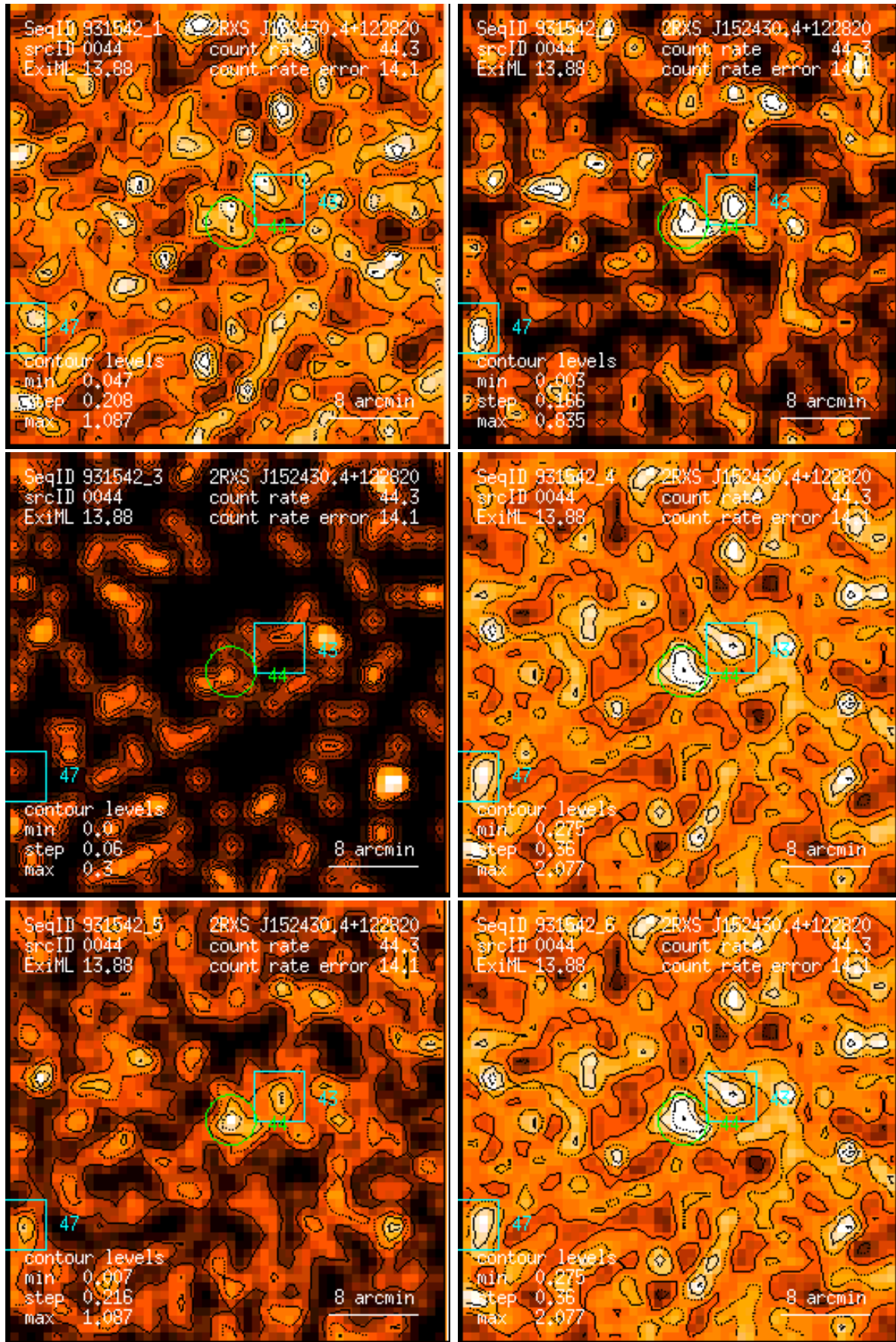
Figure 44: RASS 931542: detection 0044: band rate images, Gaussian filter: (1) PSPC channels 11 – 41, (2) 52 – 90, (3) 91 – 201, (4) 11 – 235, (5) 52 – 201, (6) 11 – 201. Broad band rates in counts/ks. Band rate contour levels in counts/ks/arcmin 2 .
