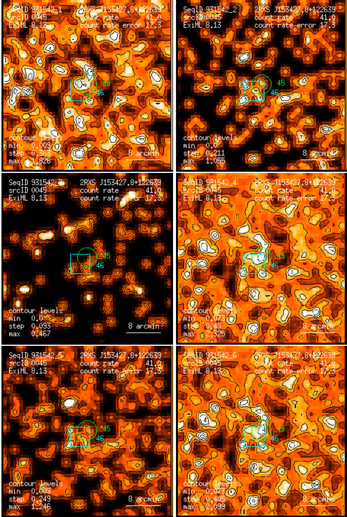
Figure 45: RASS 931542: detection 0045: band rate images, Gaussian filter: (1) PSPC channels 11 – 41, (2) 52 – 90, (3) 91 – 201, (4) 11 – 235, (5) 52 – 201, (6) 11 – 201. Broad band rates in counts/ks. Band rate contour levels in counts/ks/arcmin 2 .
