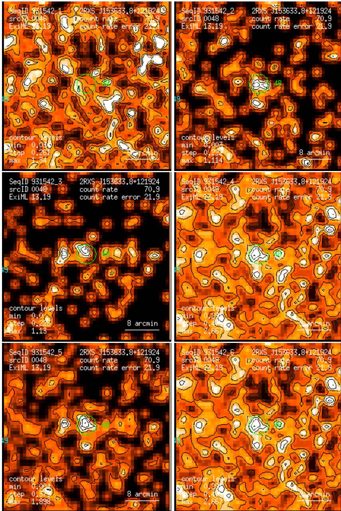
Figure 48: RASS 931542: detection 0048: band rate images, Gaussian filter: (1) PSPC channels 11 – 41, (2) 52 – 90, (3) 91 – 201, (4) 11 – 235, (5) 52 – 201, (6) 11 – 201. Broad band rates in counts/ks. Band rate contour levels in counts/ks/arcmin 2 .
