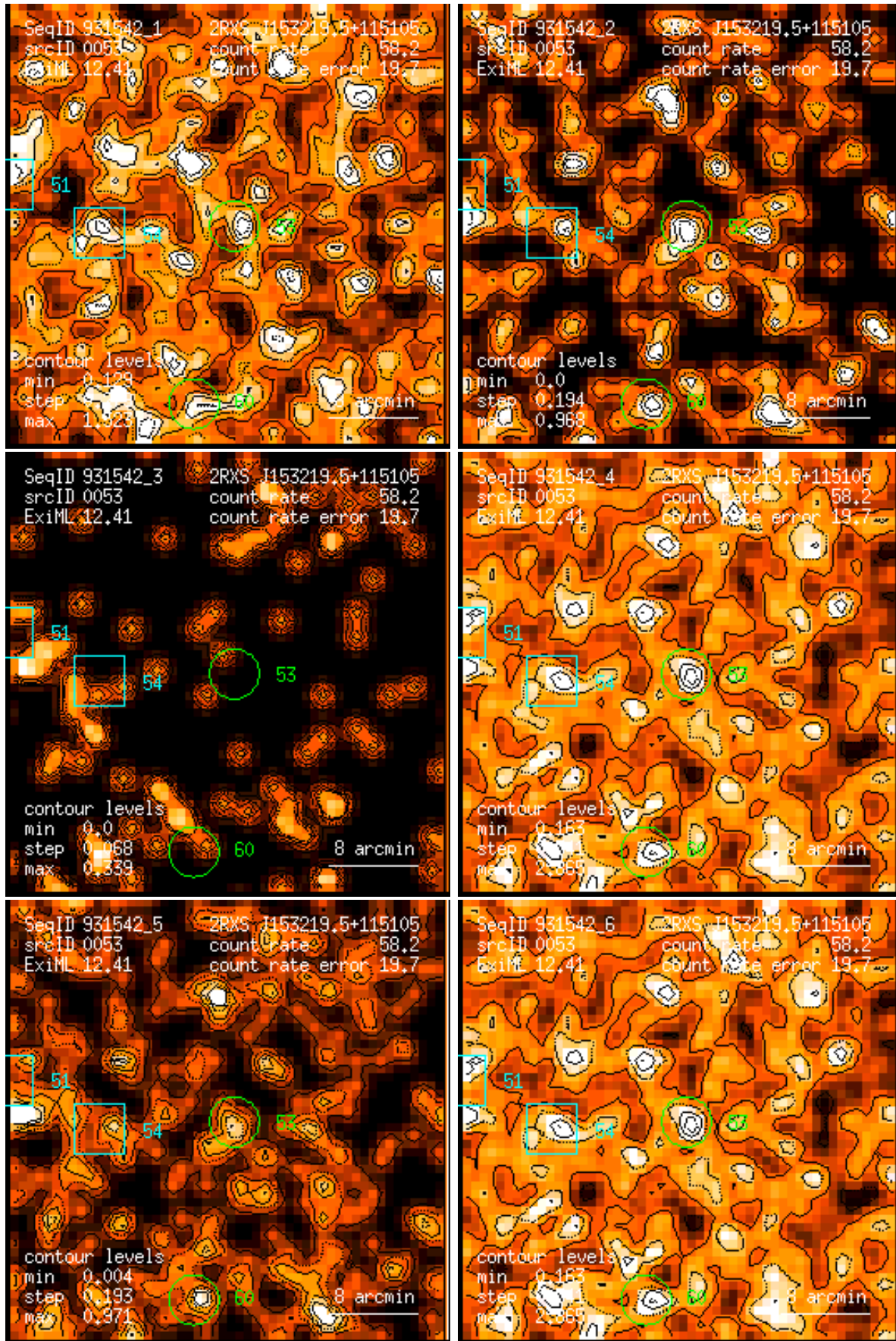
Figure 53: RASS 931542: detection 0053: band rate images, Gaussian filter: (1) PSPC channels 11 – 41, (2) 52 – 90, (3) 91 – 201, (4) 11 – 235, (5) 52 – 201, (6) 11 – 201. Broad band rates in counts/ks. Band rate contour levels in counts/ks/arcmin 2 .
