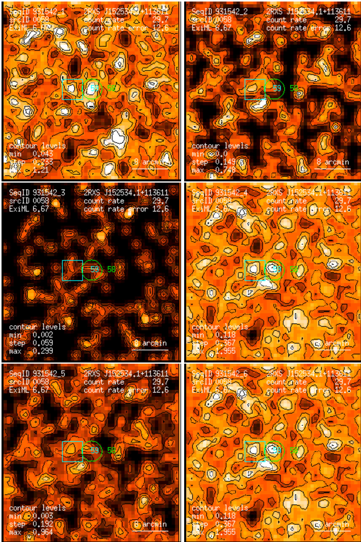
Figure 58: RASS 931542: detection 0058: band rate images, Gaussian filter: (1) PSPC channels 11 – 41, (2) 52 – 90, (3) 91 – 201, (4) 11 – 235, (5) 52 – 201, (6) 11 – 201. Broad band rates in counts/ks. Band rate contour levels in counts/ks/arcmin 2 .
