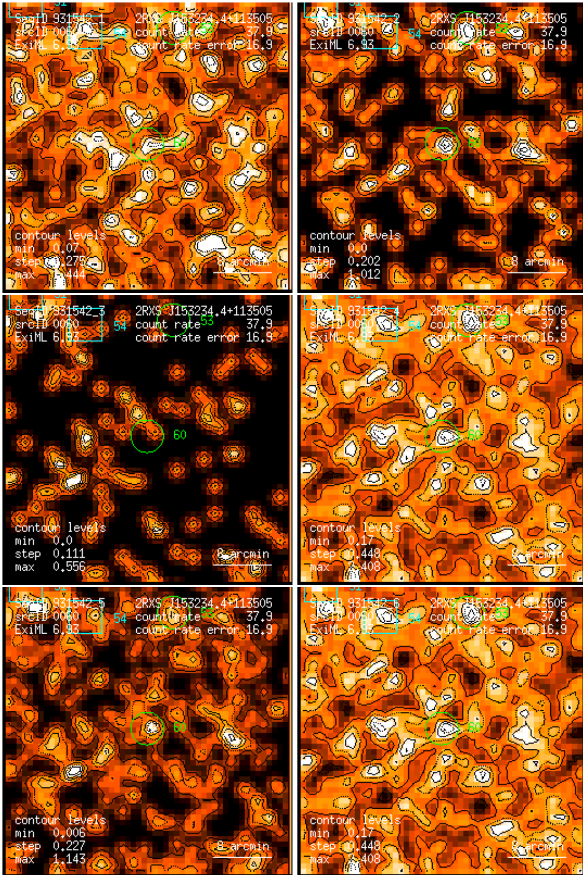
Figure 60: RASS 931542: detection 0060: band rate images, Gaussian filter: (1) PSPC channels 11 – 41, (2) 52 – 90, (3) 91 – 201, (4) 11 – 235, (5) 52 – 201, (6) 11 – 201. Broad band rates in counts/ks. Band rate contour levels in counts/ks/arcmin 2 .
