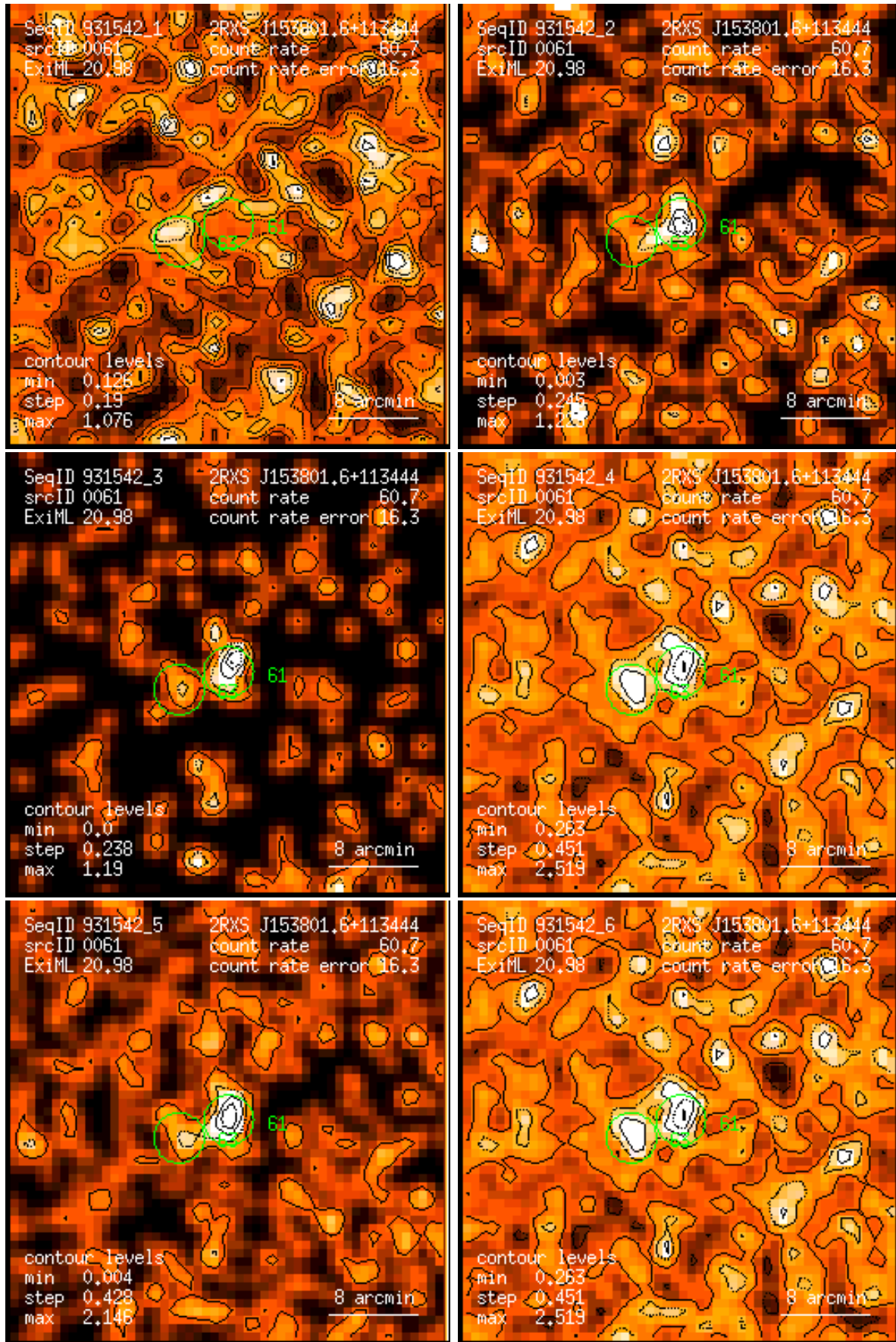
Figure 61: RASS 931542: detection 0061: band rate images, Gaussian filter: (1) PSPC channels 11 – 41, (2) 52 – 90, (3) 91 – 201, (4) 11 – 235, (5) 52 – 201, (6) 11 – 201. Broad band rates in counts/ks. Band rate contour levels in counts/ks/arcmin 2 .
