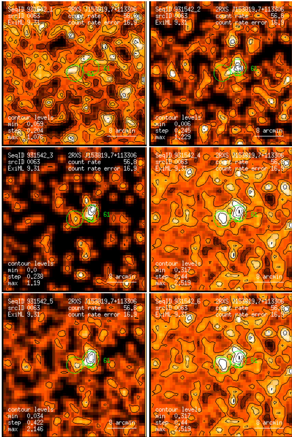
Figure 63: RASS 931542: detection 0063: band rate images, Gaussian filter: (1) PSPC channels 11 – 41, (2) 52 – 90, (3) 91 – 201, (4) 11 – 235, (5) 52 – 201, (6) 11 – 201. Broad band rates in counts/ks. Band rate contour levels in counts/ks/arcmin 2 .
