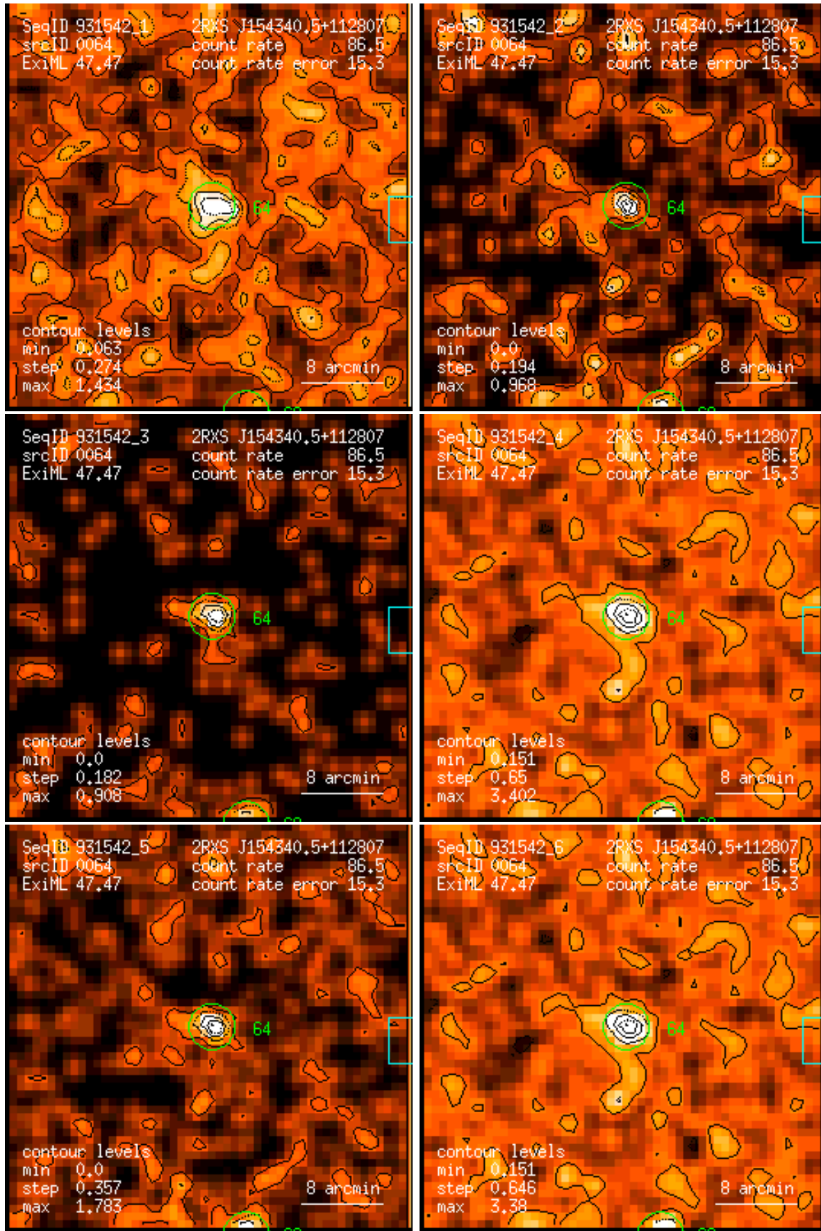
Figure 64: RASS 931542: detection 0064: band rate images, Gaussian filter: (1) PSPC channels 11 – 41, (2) 52 – 90, (3) 91 – 201, (4) 11 – 235, (5) 52 – 201, (6) 11 – 201. Broad band rates in counts/ks. Band rate contour levels in counts/ks/arcmin 2 .
