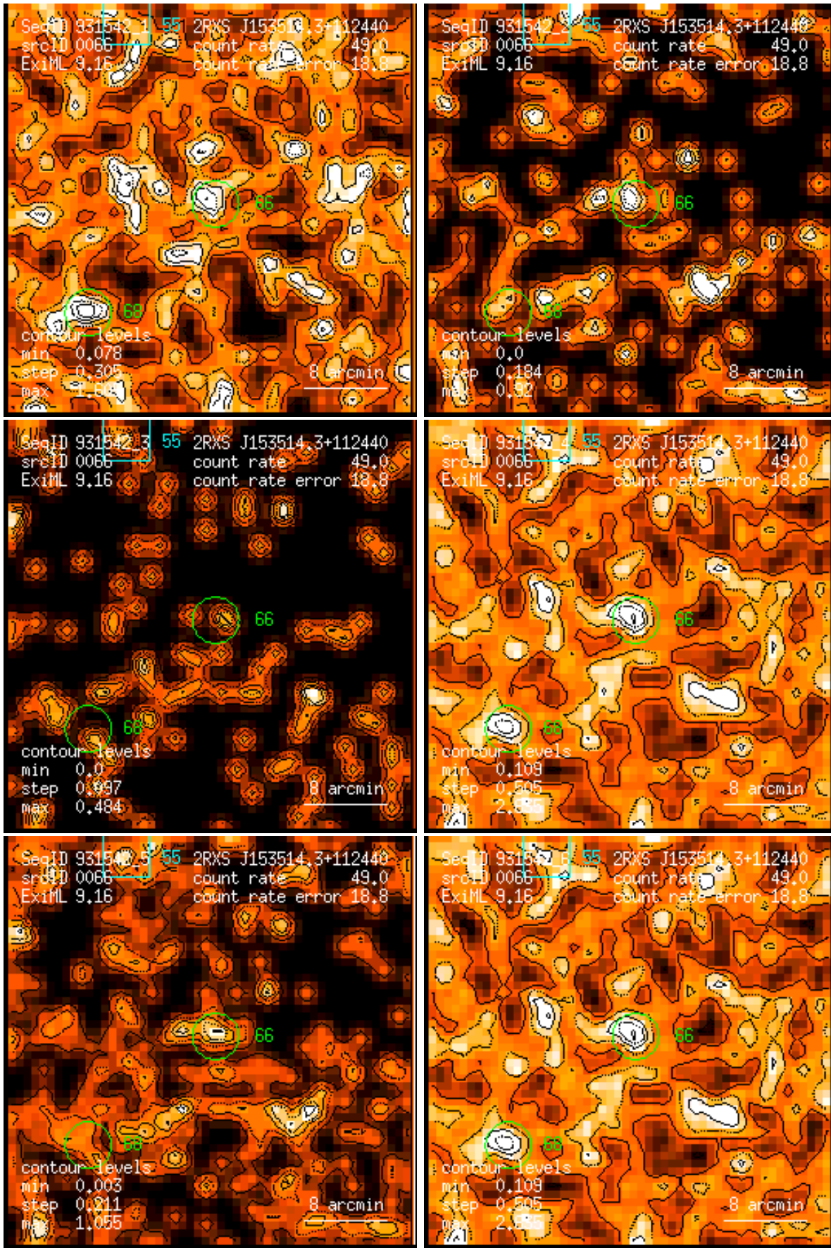
Figure 66: RASS 931542: detection 0066: band rate images, Gaussian filter: (1) PSPC channels 11 – 41, (2) 52 – 90, (3) 91 – 201, (4) 11 – 235, (5) 52 – 201, (6) 11 – 201. Broad band rates in counts/ks. Band rate contour levels in counts/ks/arcmin 2 .
