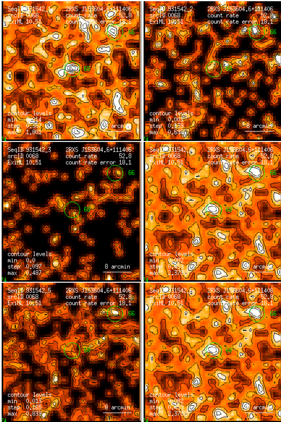
Figure 68: RASS 931542: detection 0068: band rate images, Gaussian filter: (1) PSPC channels 11 – 41, (2) 52 – 90, (3) 91 – 201, (4) 11 – 235, (5) 52 – 201, (6) 11 – 201. Broad band rates in counts/ks. Band rate contour levels in counts/ks/arcmin 2 .
