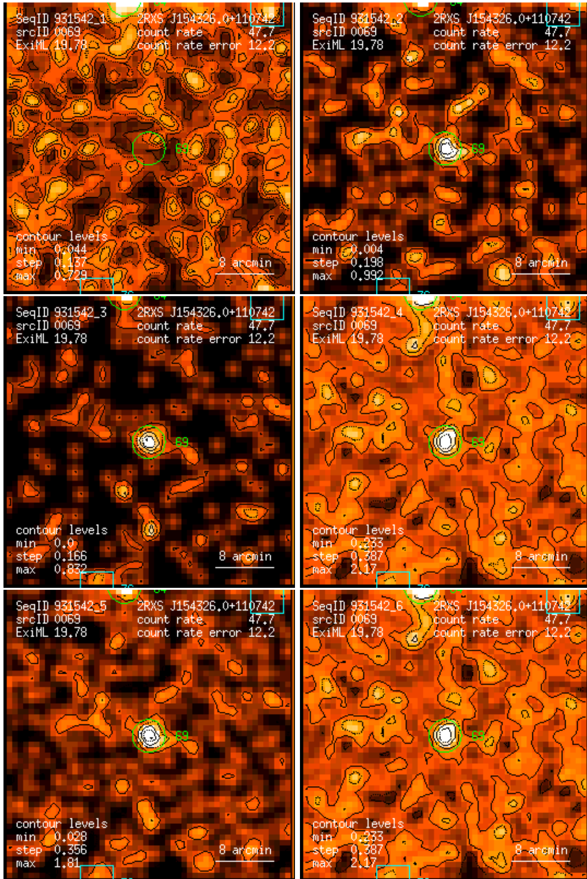
Figure 69: RASS 931542: detection 0069: band rate images, Gaussian filter: (1) PSPC channels 11 – 41, (2) 52 – 90, (3) 91 – 201, (4) 11 – 235, (5) 52 – 201, (6) 11 – 201. Broad band rates in counts/ks. Band rate contour levels in counts/ks/arcmin 2 .
