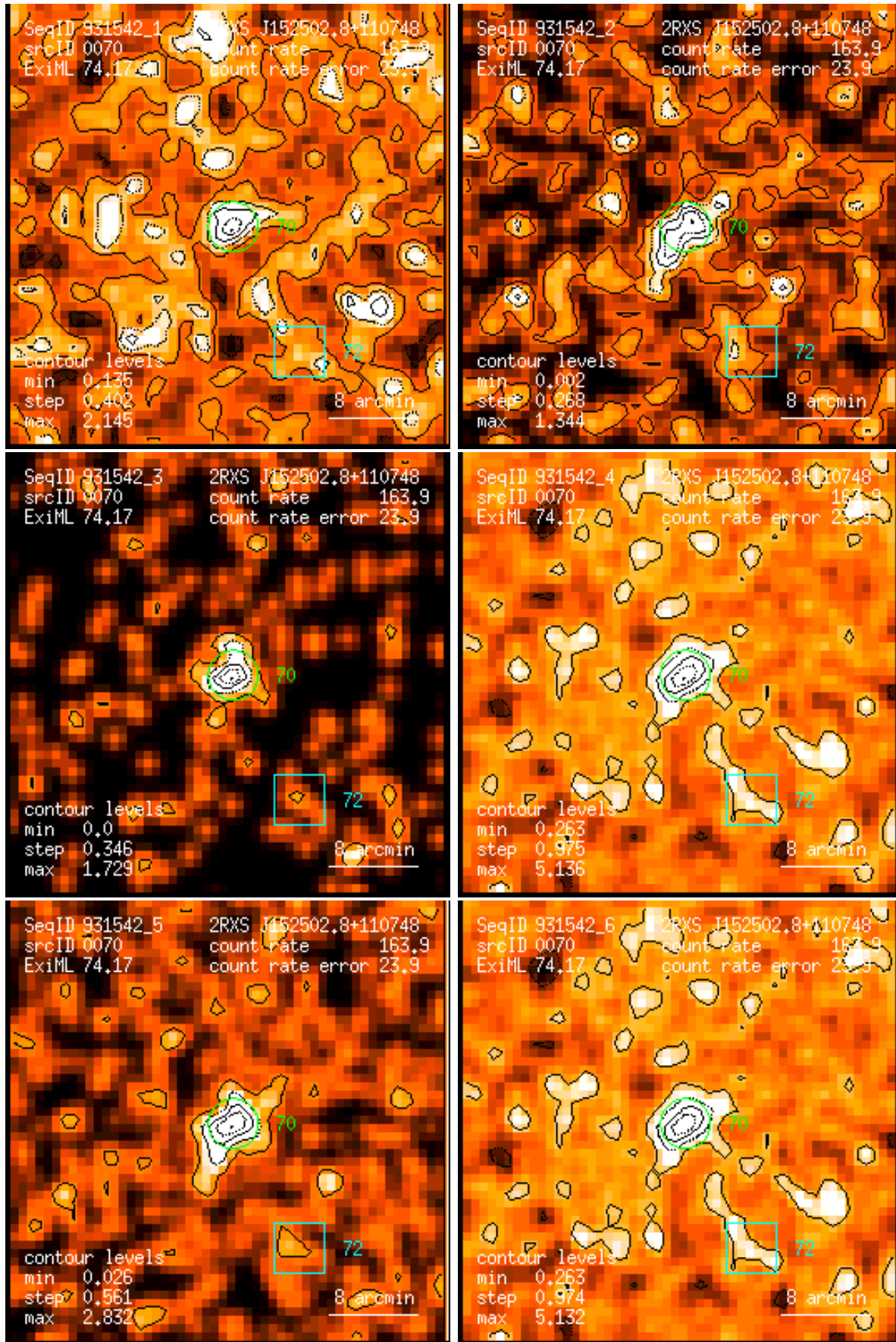
Figure 70: RASS 931542: detection 0070: band rate images, Gaussian filter: (1) PSPC channels 11 – 41, (2) 52 – 90, (3) 91 – 201, (4) 11 – 235, (5) 52 – 201, (6) 11 – 201. Broad band rates in counts/ks. Band rate contour levels in counts/ks/arcmin 2 .
