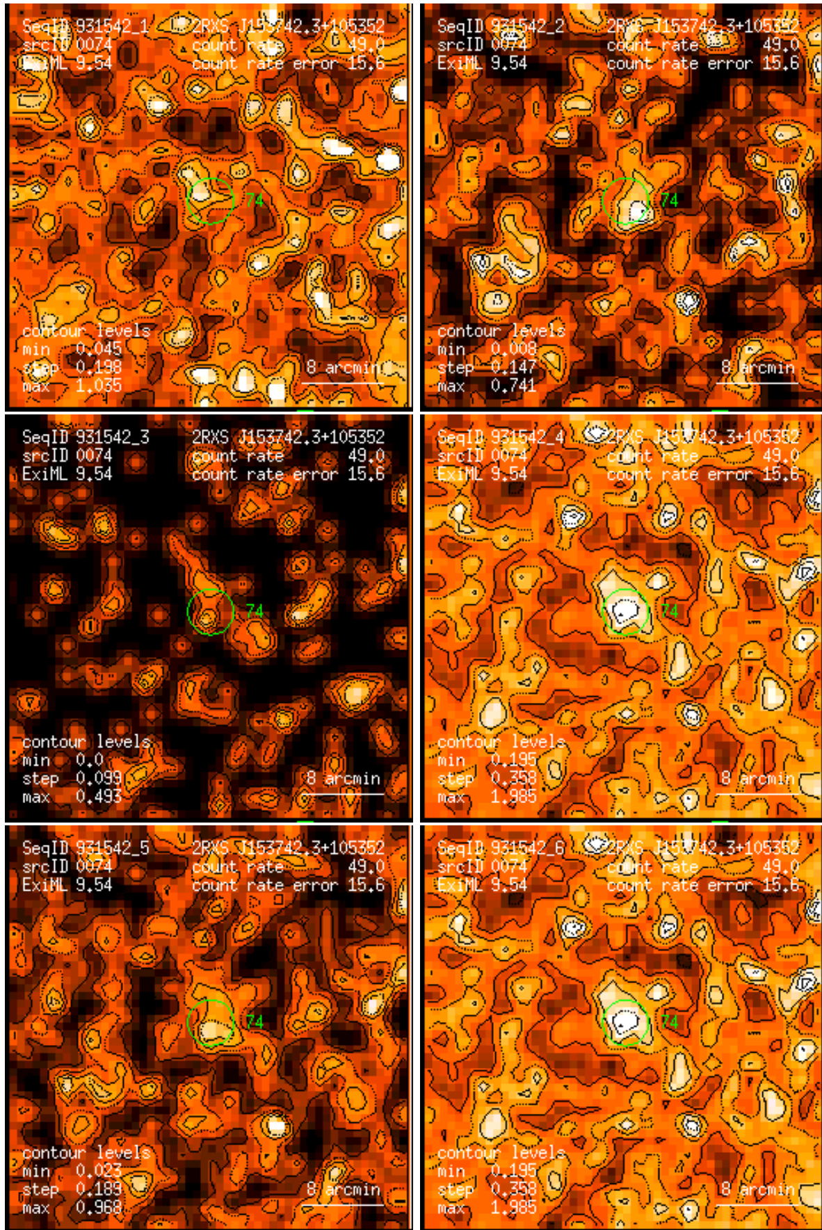
Figure 74: RASS 931542: detection 0074: band rate images, Gaussian filter: (1) PSPC channels 11 – 41, (2) 52 – 90, (3) 91 – 201, (4) 11 – 235, (5) 52 – 201, (6) 11 – 201. Broad band rates in counts/ks. Band rate contour levels in counts/ks/arcmin 2 .
