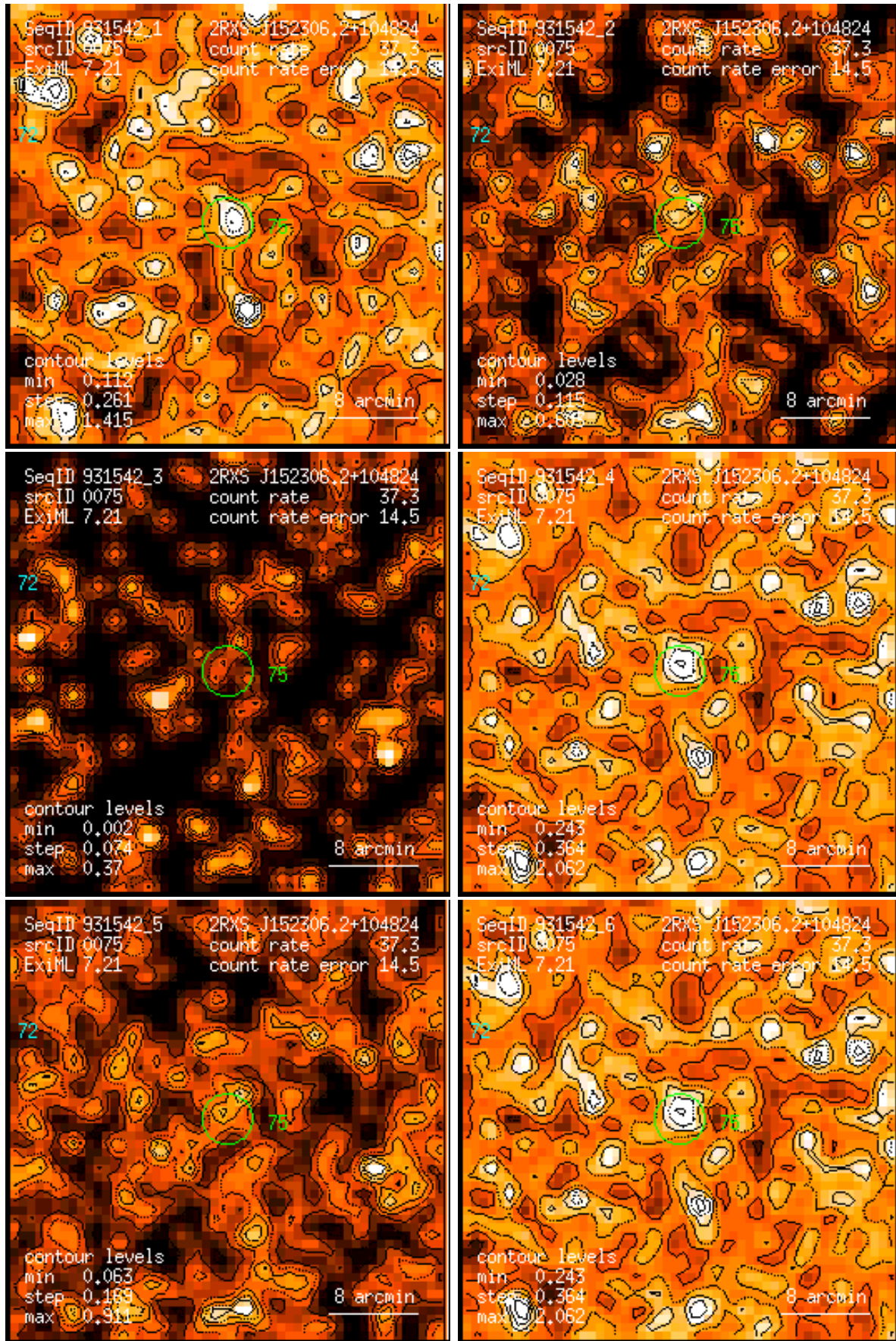
Figure 75: RASS 931542: detection 0075: band rate images, Gaussian filter: (1) PSPC channels 11 – 41, (2) 52 – 90, (3) 91 – 201, (4) 11 – 235, (5) 52 – 201, (6) 11 – 201. Broad band rates in counts/ks. Band rate contour levels in counts/ks/arcmin 2 .
