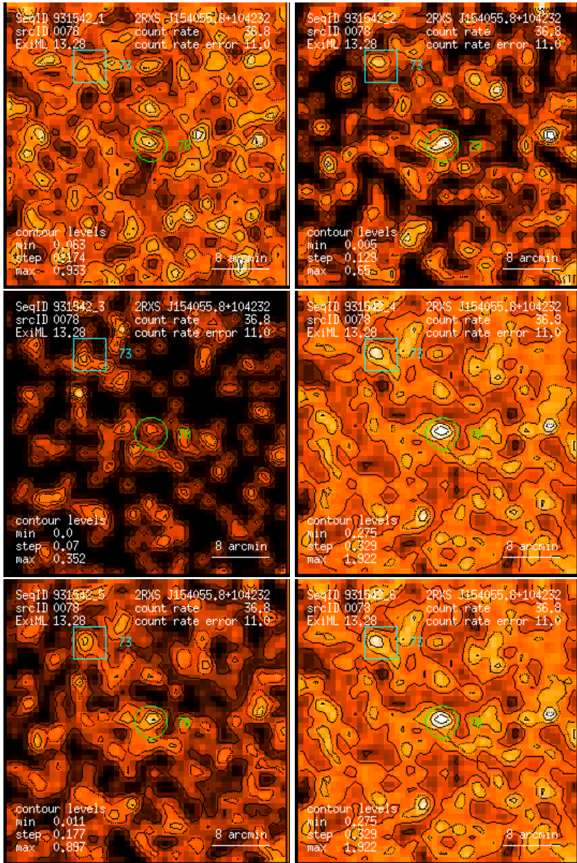
Figure 78: RASS 931542: detection 0078: band rate images, Gaussian filter: (1) PSPC channels 11 – 41, (2) 52 – 90, (3) 91 – 201, (4) 11 – 235, (5) 52 – 201, (6) 11 – 201. Broad band rates in counts/ks. Band rate contour levels in counts/ks/arcmin 2 .
