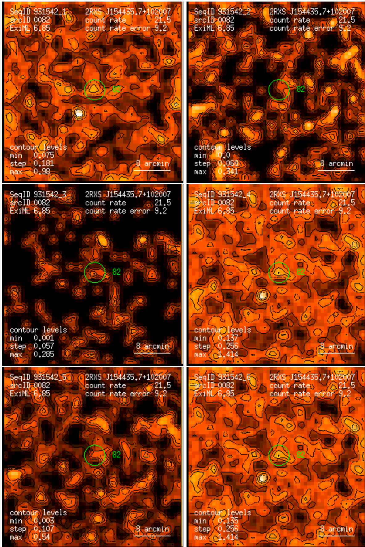
Figure 82: RASS 931542: detection 0082: band rate images, Gaussian filter: (1) PSPC channels 11 – 41, (2) 52 – 90, (3) 91 – 201, (4) 11 – 235, (5) 52 – 201, (6) 11 – 201. Broad band rates in counts/ks. Band rate contour levels in counts/ks/arcmin 2 .
