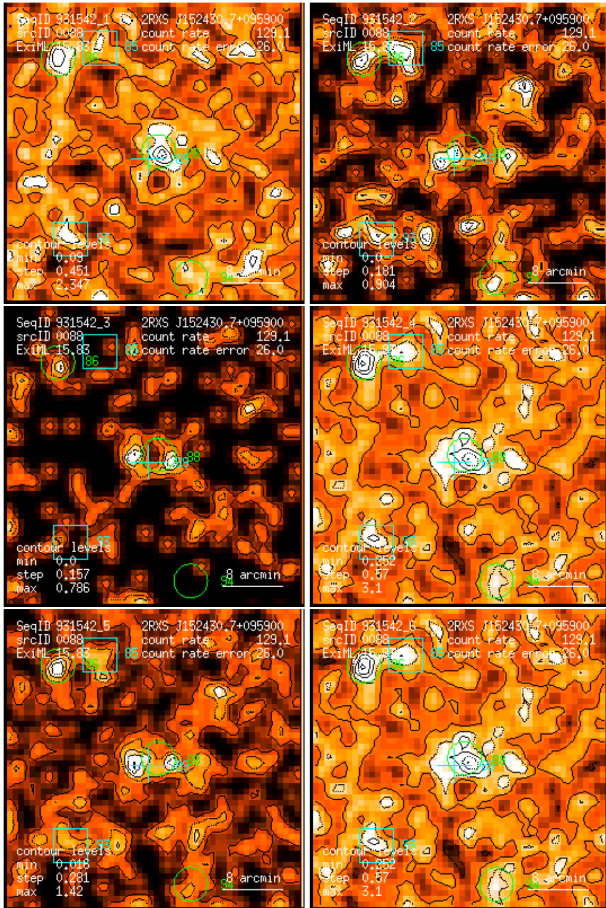
Figure 88: RASS 931542: detection 0088: band rate images, Gaussian filter: (1) PSPC channels 11 – 41, (2) 52 – 90, (3) 91 – 201, (4) 11 – 235, (5) 52 – 201, (6) 11 – 201. Broad band rates in counts/ks. Band rate contour levels in counts/ks/arcmin 2 .
