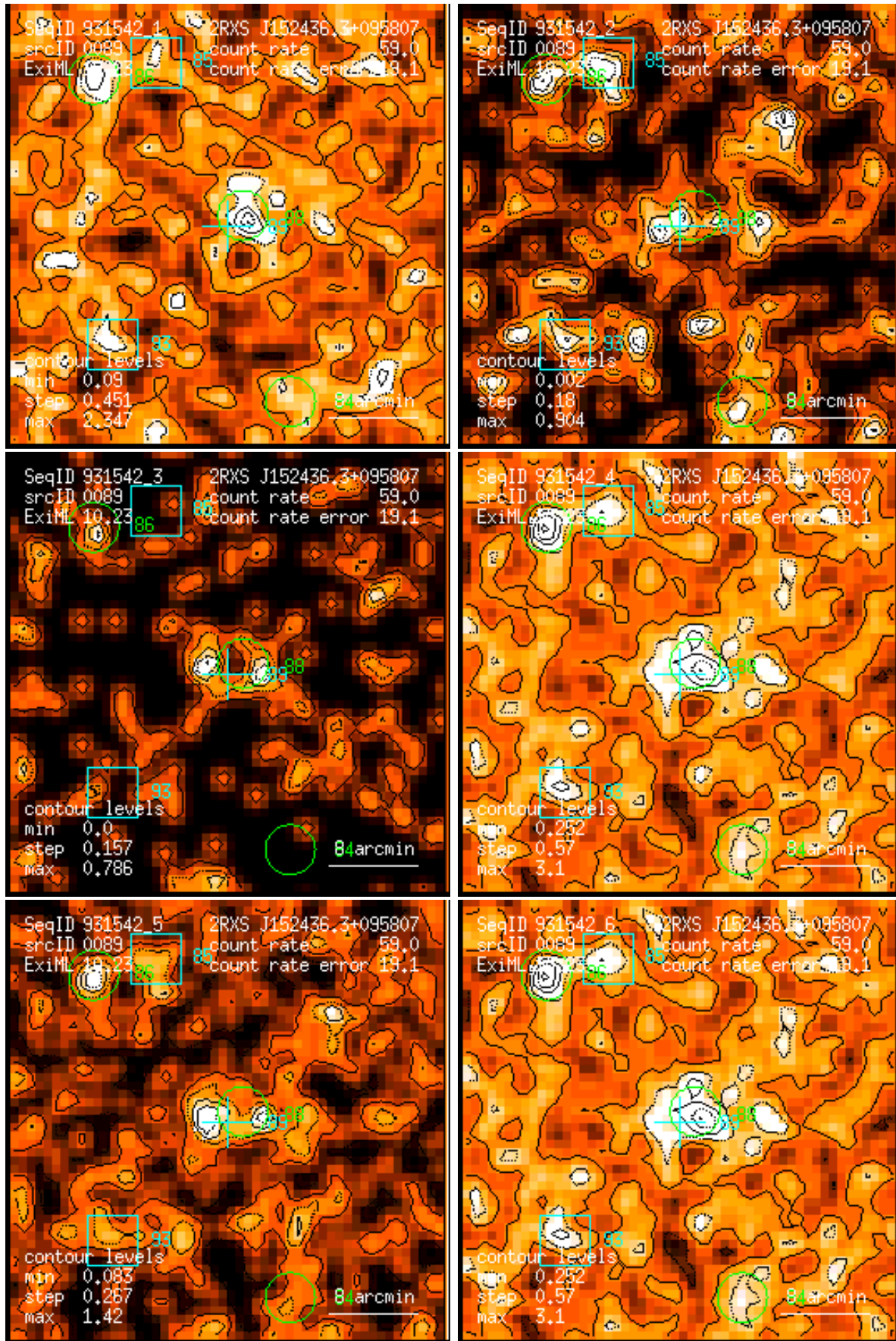
Figure 89: RASS 931542: detection 0089: band rate images, Gaussian filter: (1) PSPC channels 11 – 41, (2) 52 – 90, (3) 91 – 201, (4) 11 – 235, (5) 52 – 201, (6) 11 – 201. Broad band rates in counts/ks. Band rate contour levels in counts/ks/arcmin 2 .
