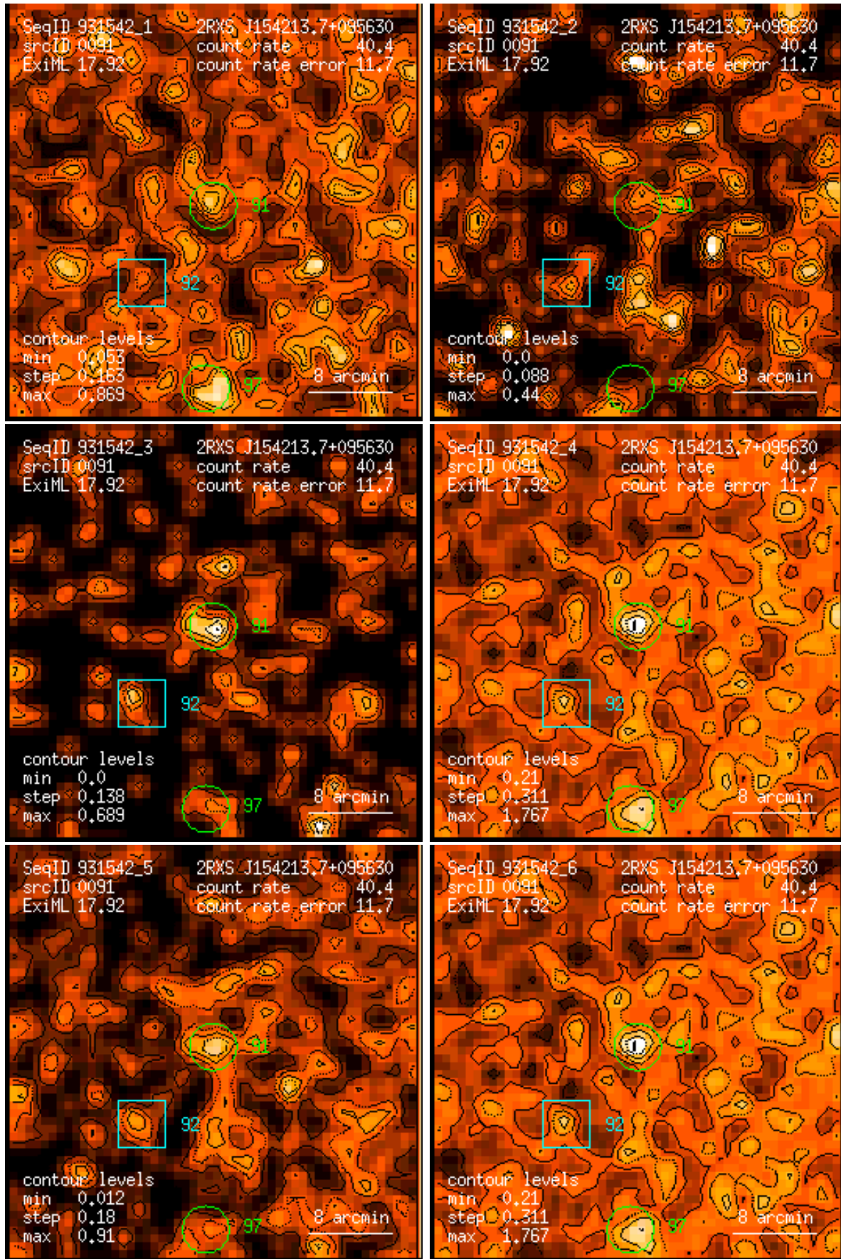
Figure 91: RASS 931542: detection 0091: band rate images, Gaussian filter: (1) PSPC channels 11 – 41, (2) 52 – 90, (3) 91 – 201, (4) 11 – 235, (5) 52 – 201, (6) 11 – 201. Broad band rates in counts/ks. Band rate contour levels in counts/ks/arcmin 2 .
