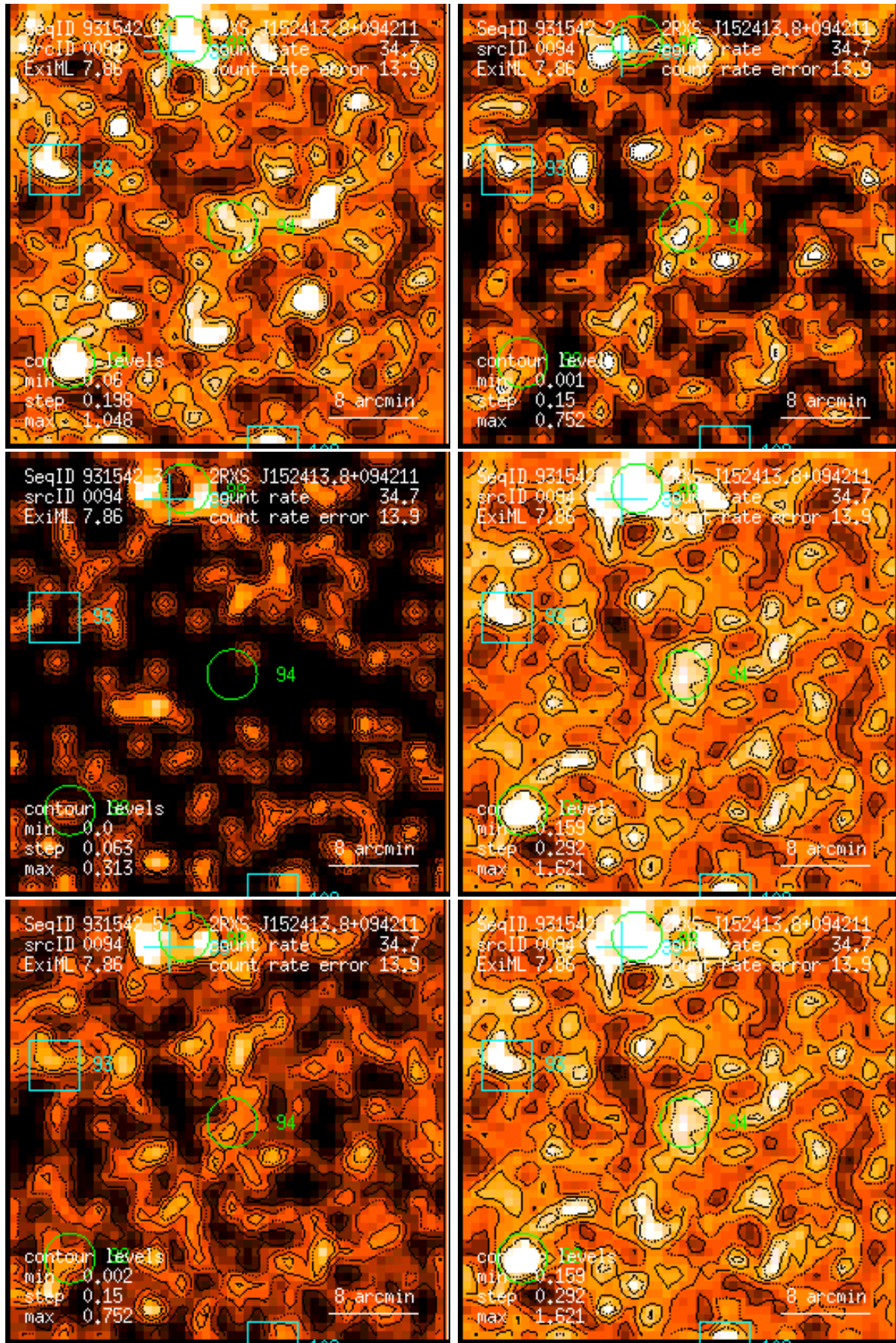
Figure 94: RASS 931542: detection 0094: band rate images, Gaussian filter: (1) PSPC channels 11 – 41, (2) 52 – 90, (3) 91 – 201, (4) 11 – 235, (5) 52 – 201, (6) 11 – 201. Broad band rates in counts/ks. Band rate contour levels in counts/ks/arcmin 2 .
