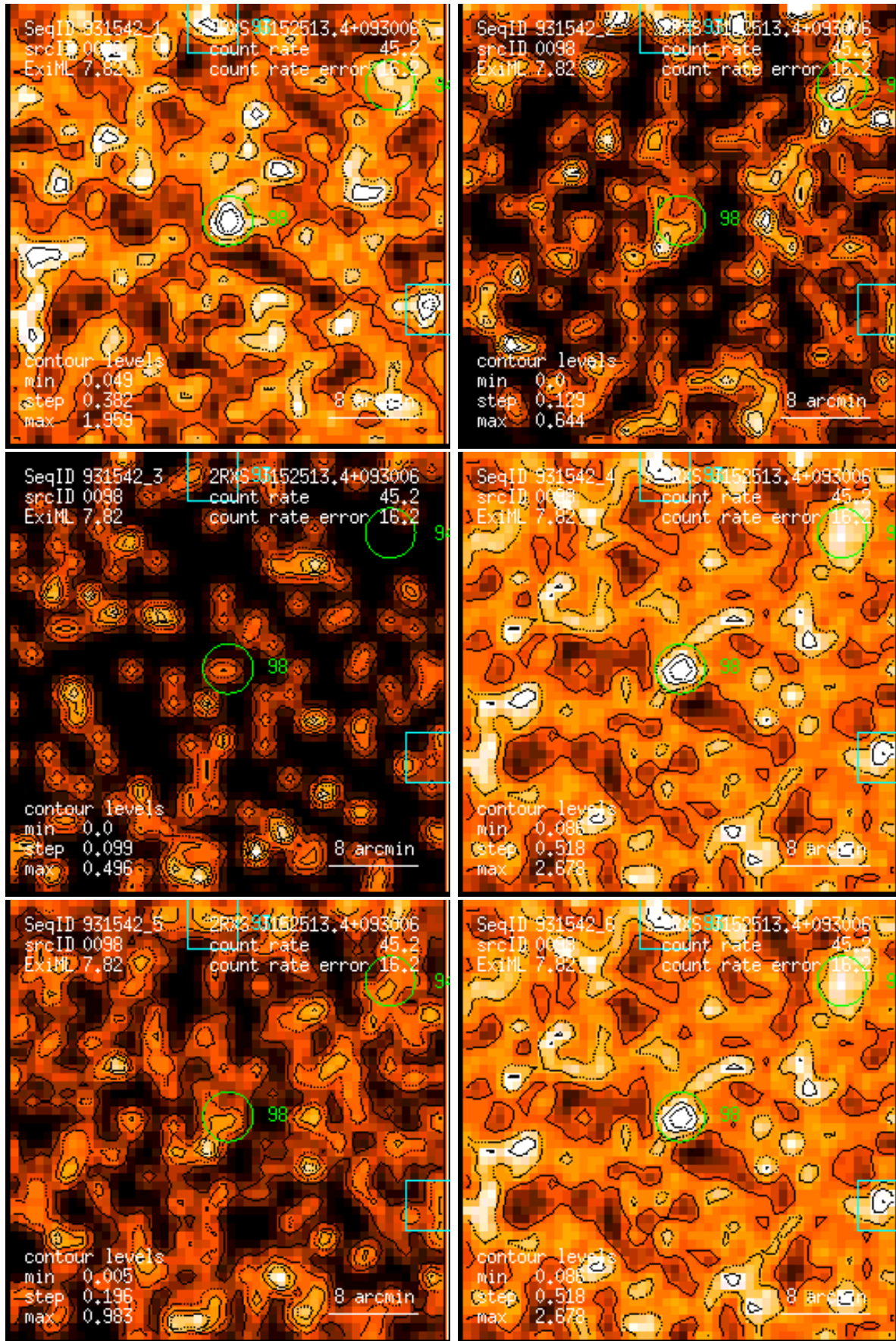
Figure 98: RASS 931542: detection 0098: band rate images, Gaussian filter: (1) PSPC channels 11 – 41, (2) 52 – 90, (3) 91 – 201, (4) 11 – 235, (5) 52 – 201, (6) 11 – 201. Broad band rates in counts/ks. Band rate contour levels in counts/ks/arcmin 2 .
