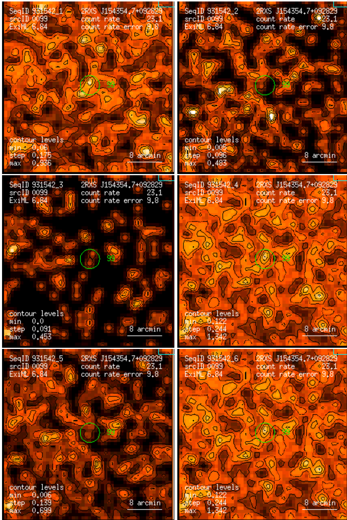
Figure 99: RASS 931542: detection 0099: band rate images, Gaussian filter: (1) PSPC channels 11 – 41, (2) 52 – 90, (3) 91 – 201, (4) 11 – 235, (5) 52 – 201, (6) 11 – 201. Broad band rates in counts/ks. Band rate contour levels in counts/ks/arcmin 2 .
