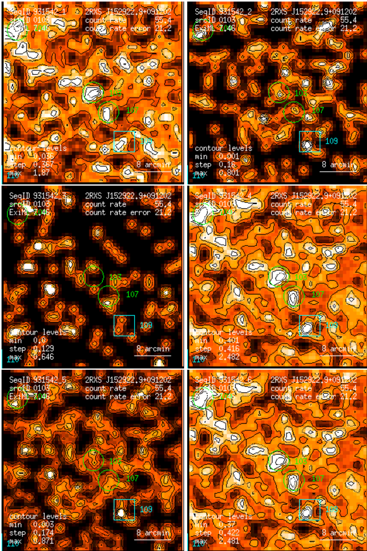
Figure 103: RASS 931542: detection 0103: band rate images, Gaussian filter: (1) PSPC channels 11 – 41, (2) 52 – 90, (3) 91 – 201, (4) 11 – 235, (5) 52 – 201, (6) 11 – 201. Broad band rates in counts/ks. Band rate contour levels in counts/ks/arcmin 2 .
