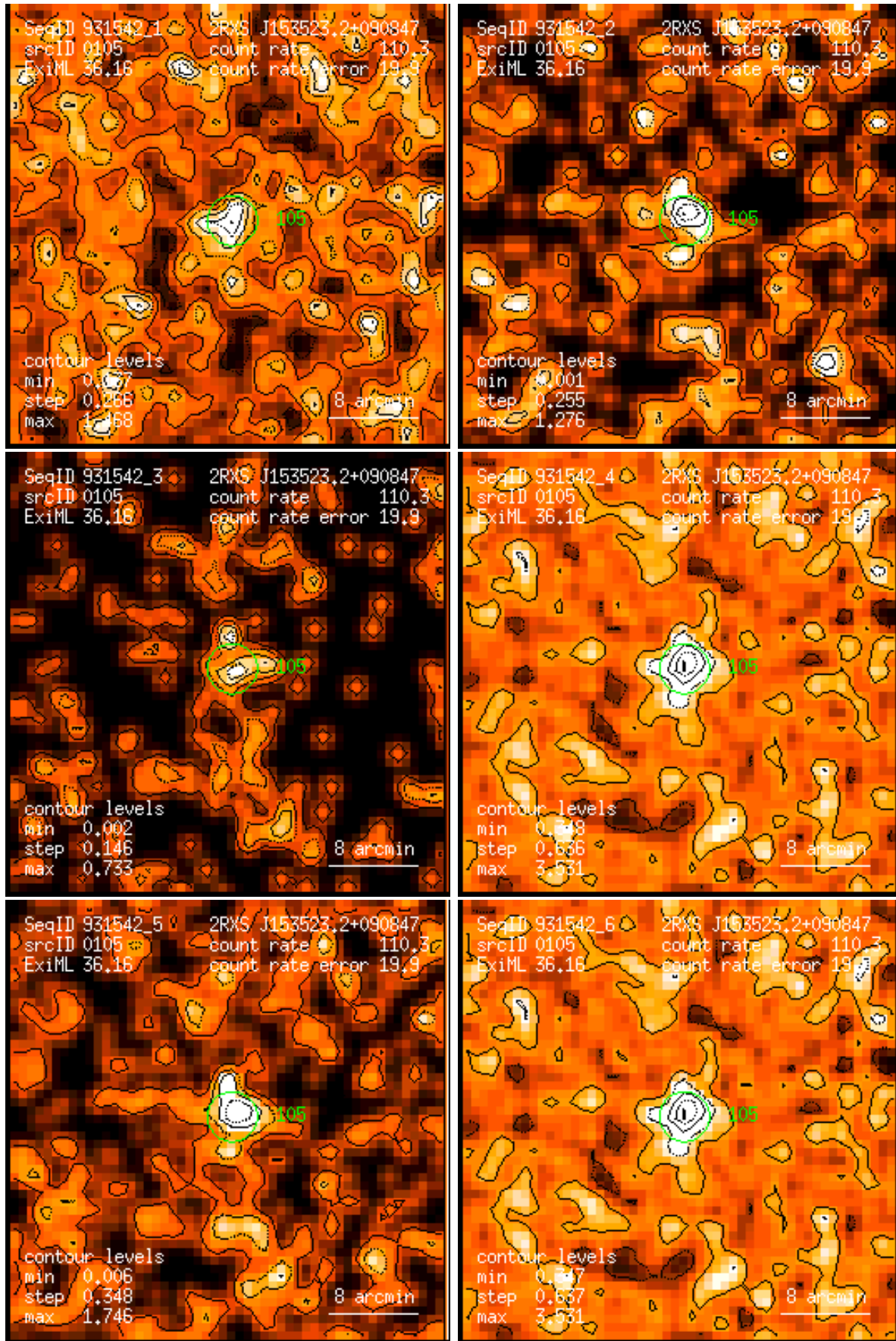
Figure 105: RASS 931542: detection 0105: band rate images, Gaussian filter: (1) PSPC channels 11 – 41, (2) 52 – 90, (3) 91 – 201, (4) 11 – 235, (5) 52 – 201, (6) 11 – 201. Broad band rates in counts/ks. Band rate contour levels in counts/ks/arcmin 2 .
