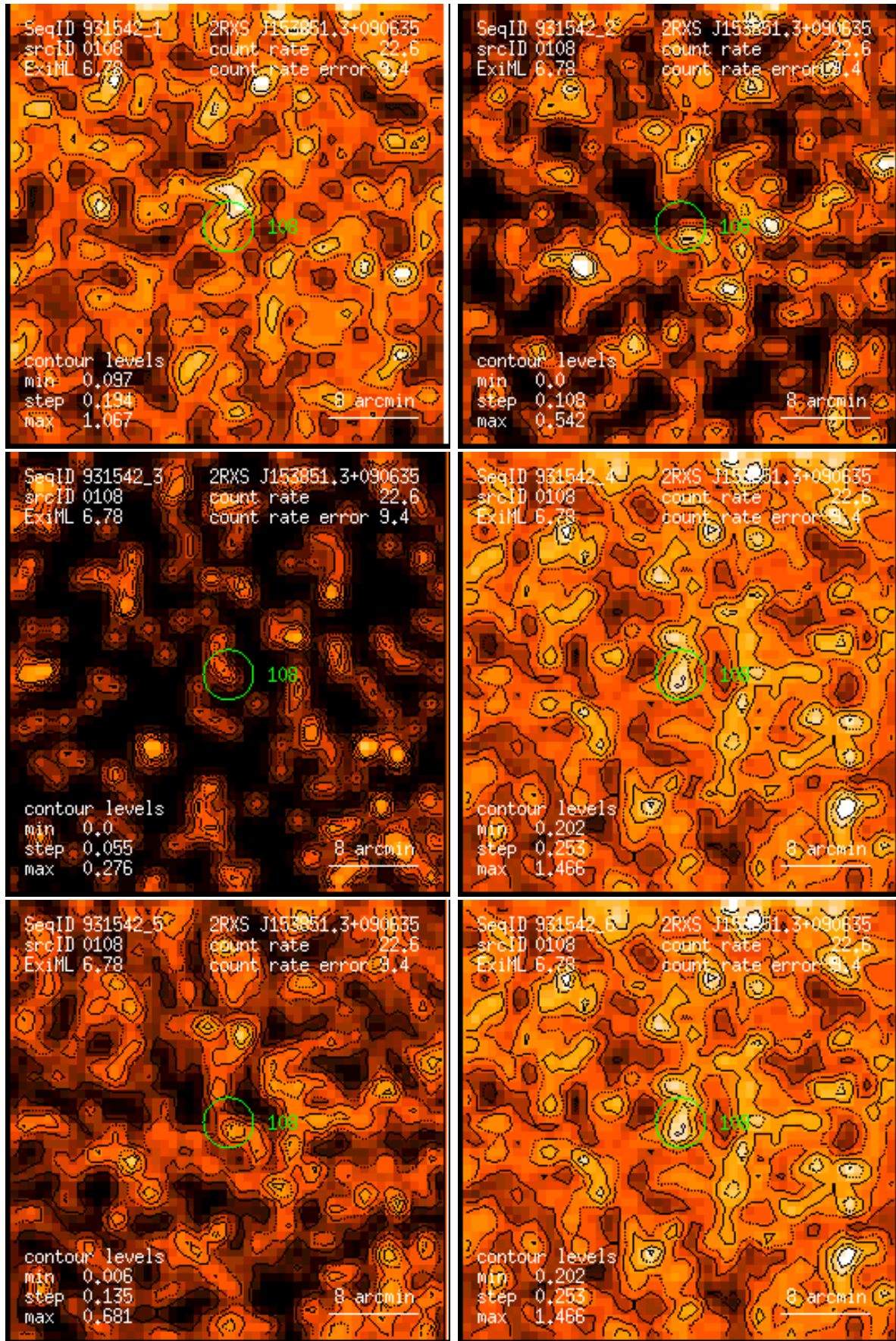
Figure 108: RASS 931542: detection 0108: band rate images, Gaussian filter: (1) PSPC channels 11 – 41, (2) 52 – 90, (3) 91 – 201, (4) 11 – 235, (5) 52 – 201, (6) 11 – 201. Broad band rates in counts/ks. Band rate contour levels in counts/ks/arcmin 2 .
