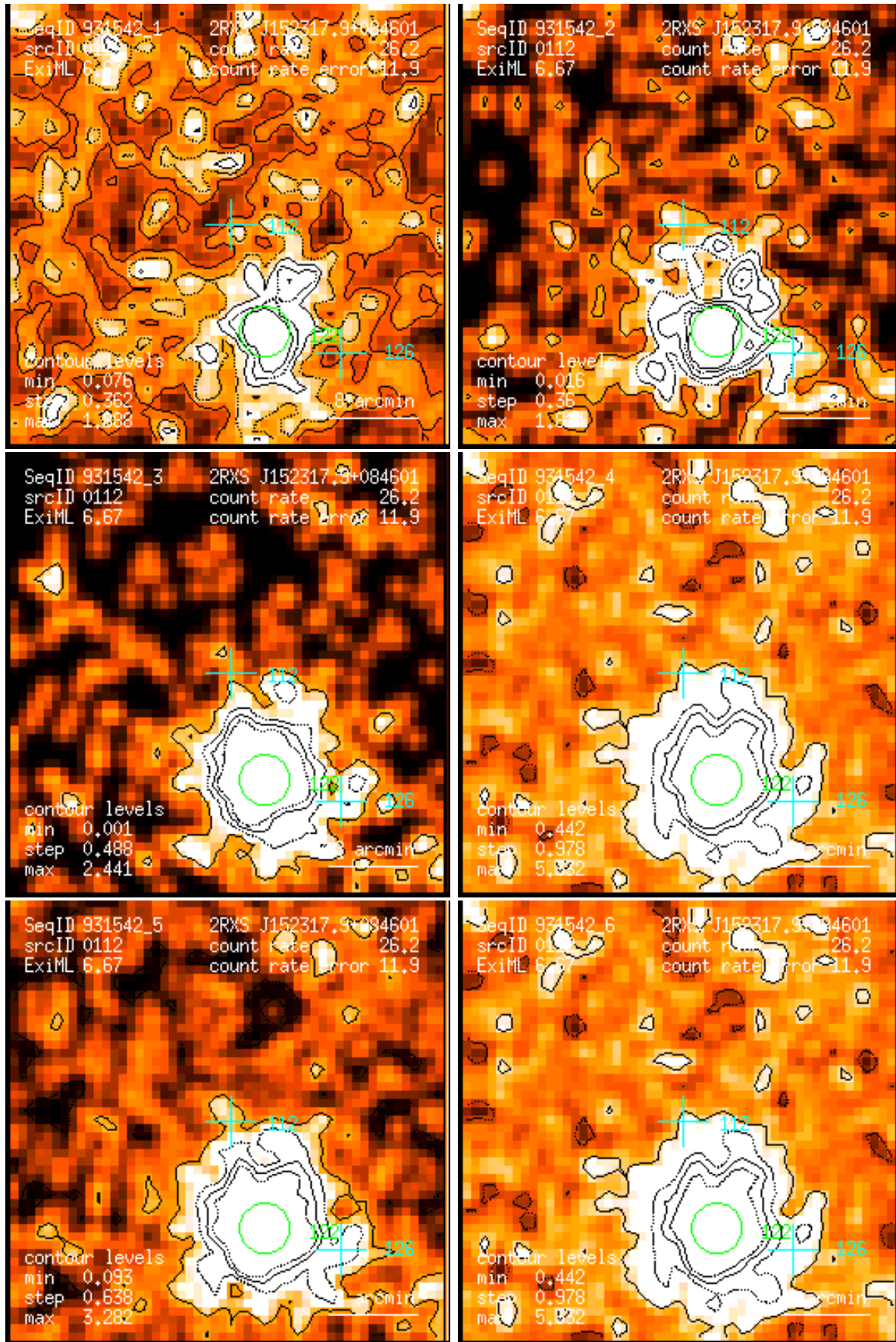
Figure 112: RASS 931542: detection 0112: band rate images, Gaussian filter: (1) PSPC channels 11 – 41, (2) 52 – 90, (3) 91 – 201, (4) 11 – 235, (5) 52 – 201, (6) 11 – 201. Broad band rates in counts/ks. Band rate contour levels in counts/ks/arcmin 2 .
