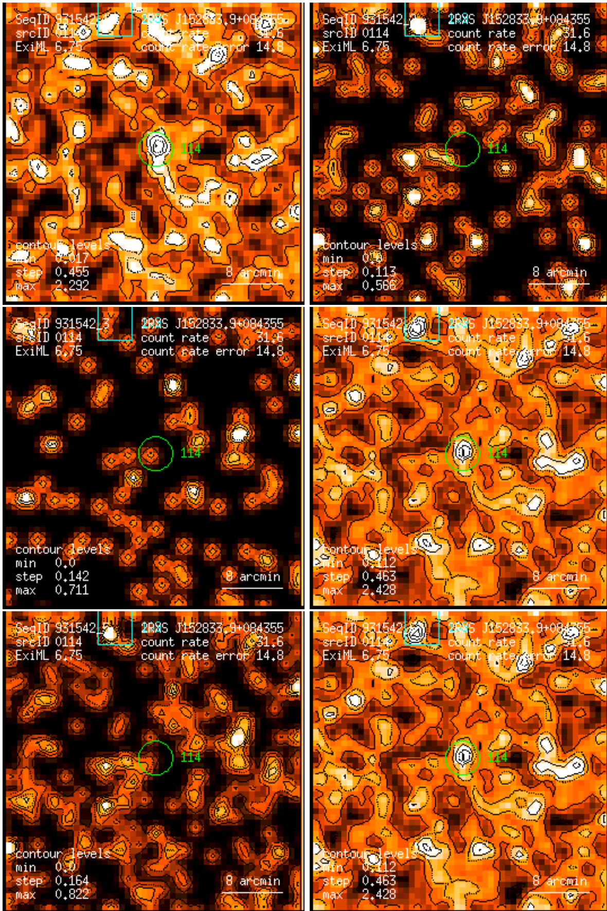
Figure 114: RASS 931542: detection 0114: band rate images, Gaussian filter: (1) PSPC channels 11 – 41, (2) 52 – 90, (3) 91 – 201, (4) 11 – 235, (5) 52 – 201, (6) 11 – 201. Broad band rates in counts/ks. Band rate contour levels in counts/ks/arcmin 2 .
