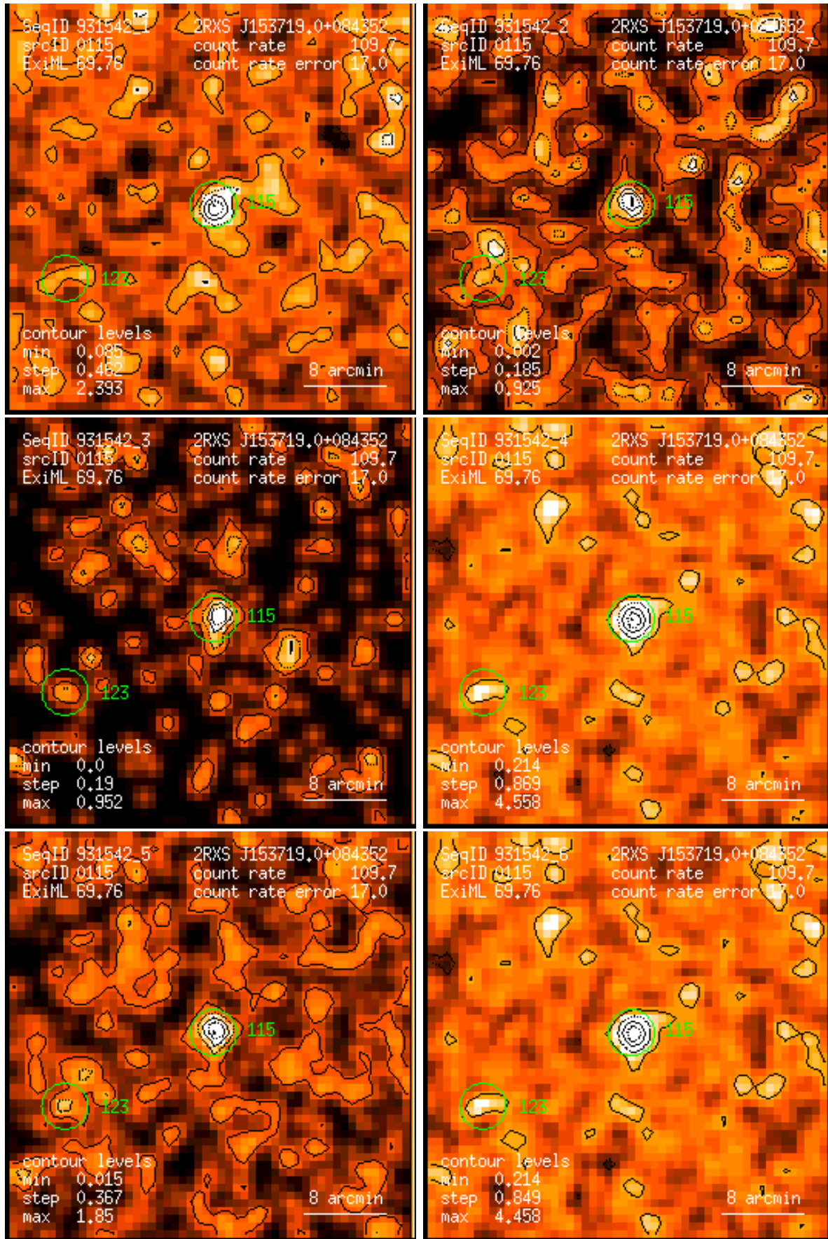
Figure 115: RASS 931542: detection 0115: band rate images, Gaussian filter: (1) PSPC channels 11 – 41, (2) 52 – 90, (3) 91 – 201, (4) 11 – 235, (5) 52 – 201, (6) 11 – 201. Broad band rates in counts/ks. Band rate contour levels in counts/ks/arcmin 2 .
