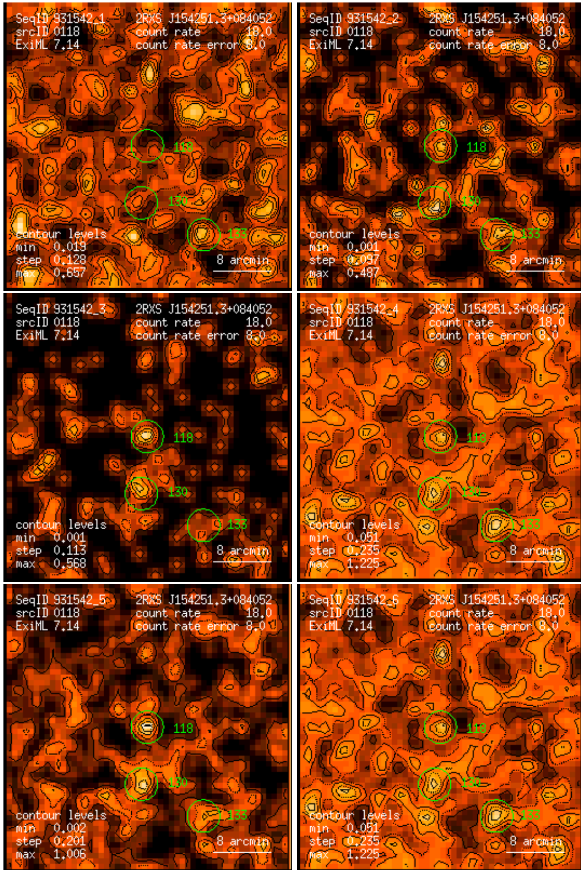
Figure 118: RASS 931542: detection 0118: band rate images, Gaussian filter: (1) PSPC channels 11 – 41, (2) 52 – 90, (3) 91 – 201, (4) 11 – 235, (5) 52 – 201, (6) 11 – 201. Broad band rates in counts/ks. Band rate contour levels in counts/ks/arcmin 2 .
