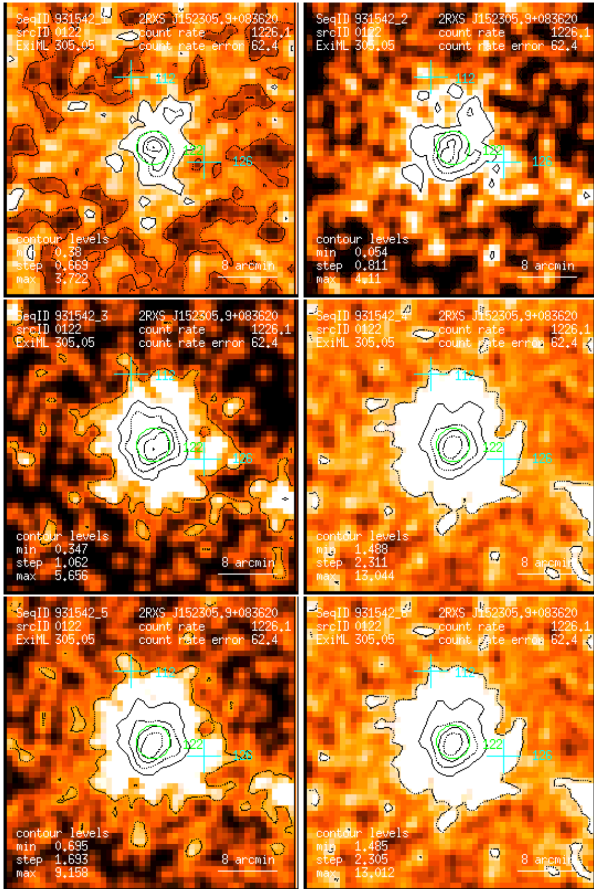
Figure 122: RASS 931542: detection 0122: band rate images, Gaussian filter: (1) PSPC channels 11 – 41, (2) 52 – 90, (3) 91 – 201, (4) 11 – 235, (5) 52 – 201, (6) 11 – 201. Broad band rates in counts/ks. Band rate contour levels in counts/ks/arcmin 2 .
