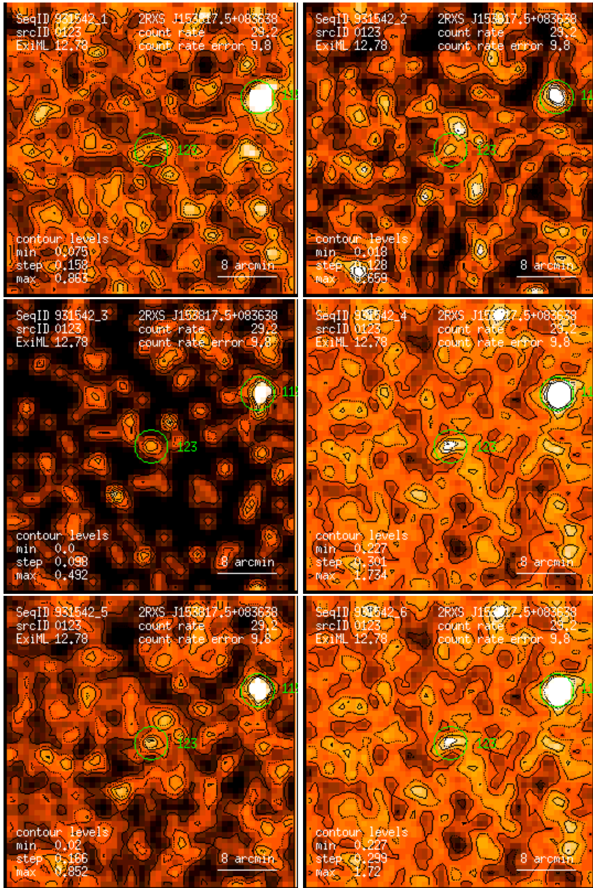
Figure 123: RASS 931542: detection 0123: band rate images, Gaussian filter: (1) PSPC channels 11 – 41, (2) 52 – 90, (3) 91 – 201, (4) 11 – 235, (5) 52 – 201, (6) 11 – 201. Broad band rates in counts/ks. Band rate contour levels in counts/ks/arcmin 2 .
