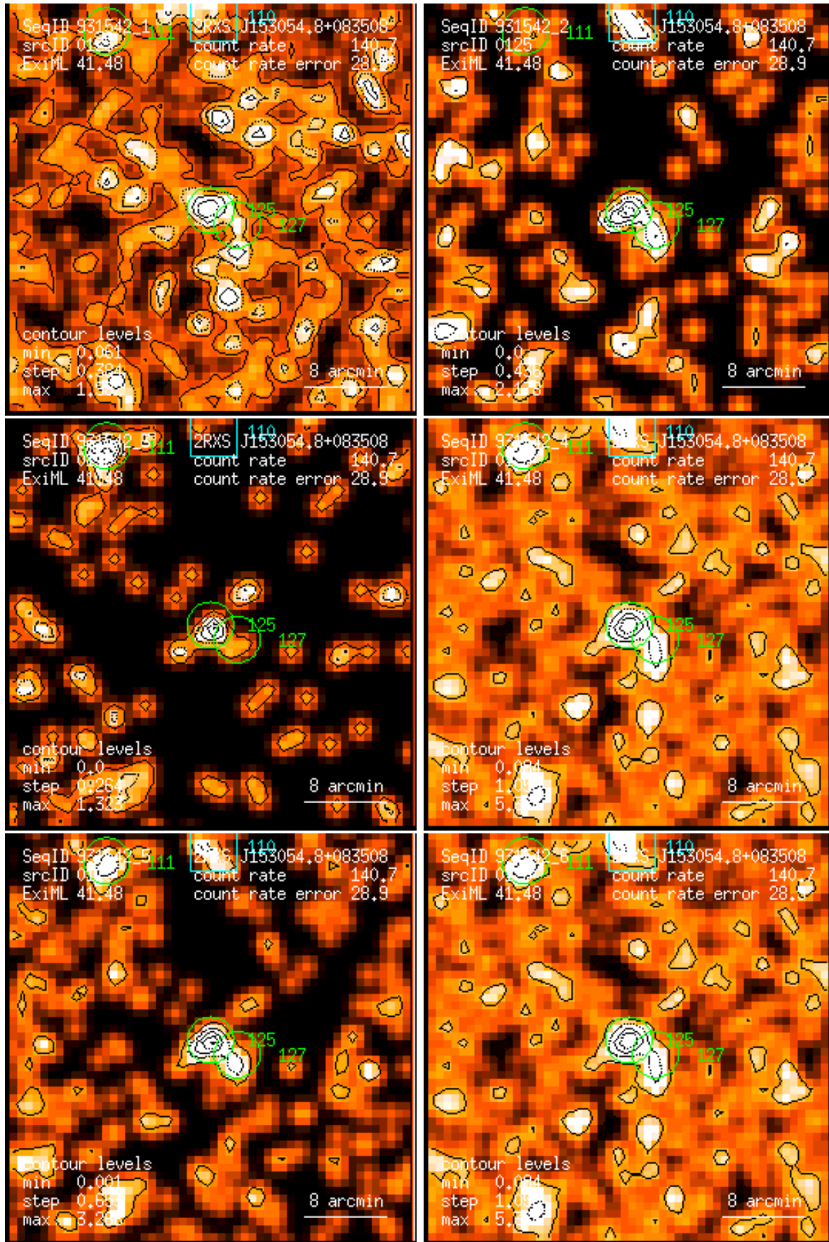
Figure 125: RASS 931542: detection 0125: band rate images, Gaussian filter: (1) PSPC channels 11 – 41, (2) 52 – 90, (3) 91 – 201, (4) 11 – 235, (5) 52 – 201, (6) 11 – 201. Broad band rates in counts/ks. Band rate contour levels in counts/ks/arcmin 2 .
