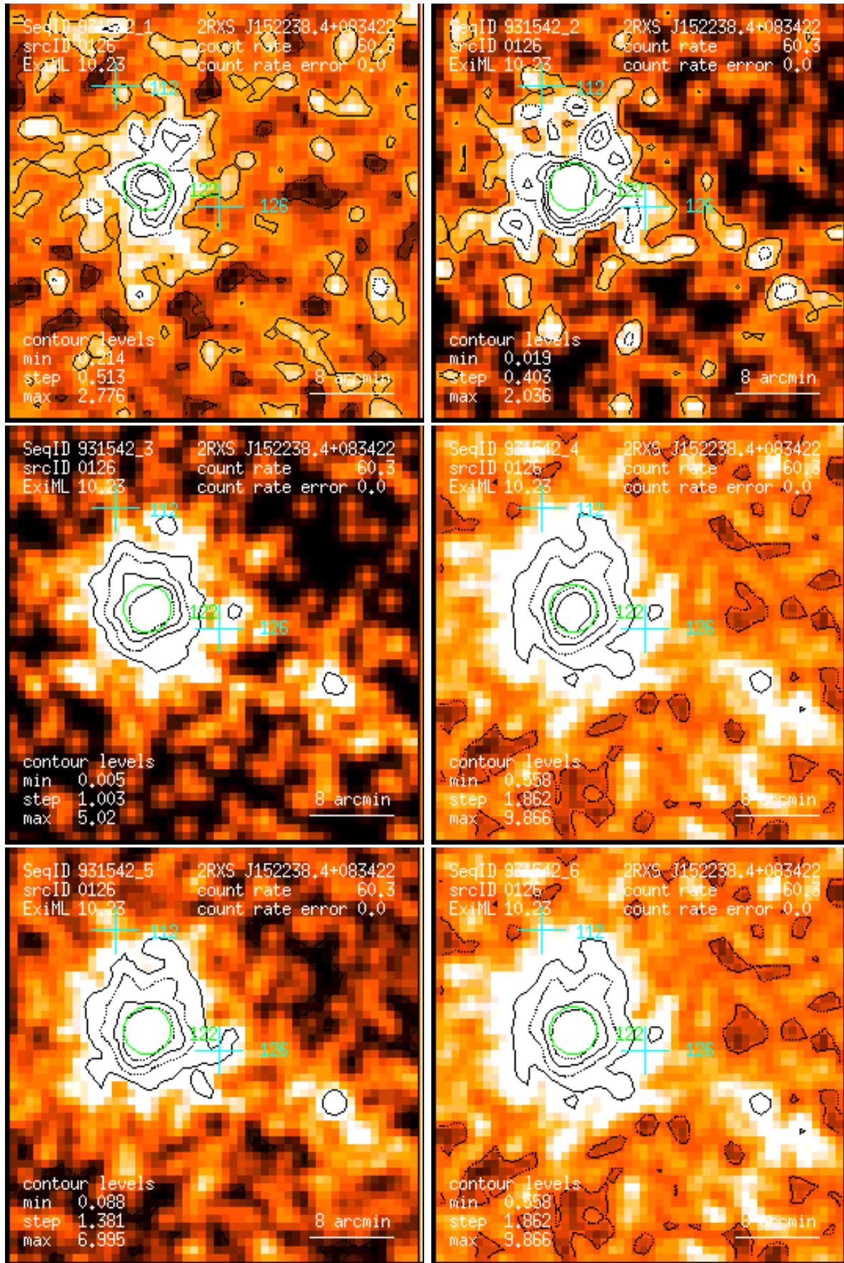
Figure 126: RASS 931542: detection 0126: band rate images, Gaussian filter: (1) PSPC channels 11 – 41, (2) 52 – 90, (3) 91 – 201, (4) 11 – 235, (5) 52 – 201, (6) 11 – 201. Broad band rates in counts/ks. Band rate contour levels in counts/ks/arcmin 2 .
