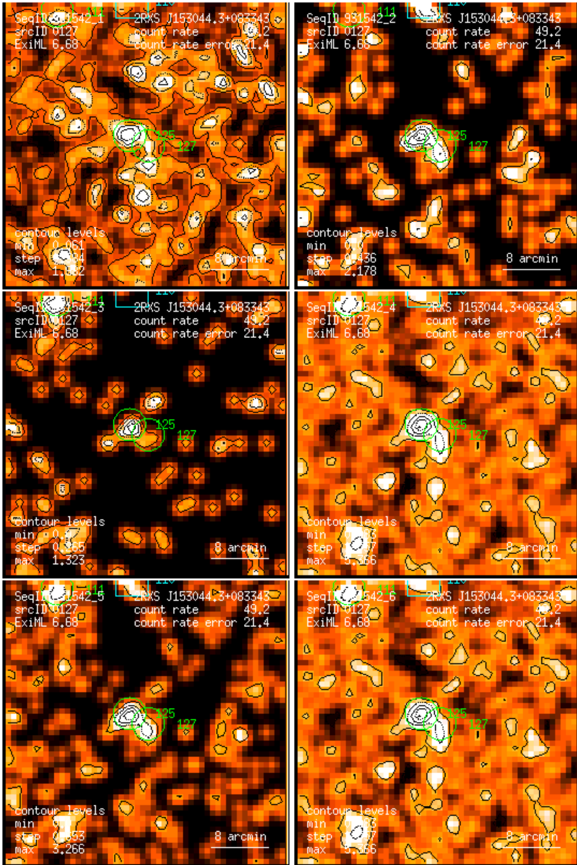
Figure 127: RASS 931542: detection 0127: band rate images, Gaussian filter: (1) PSPC channels 11 – 41, (2) 52 – 90, (3) 91 – 201, (4) 11 – 235, (5) 52 – 201, (6) 11 – 201. Broad band rates in counts/ks. Band rate contour levels in counts/ks/arcmin 2 .
