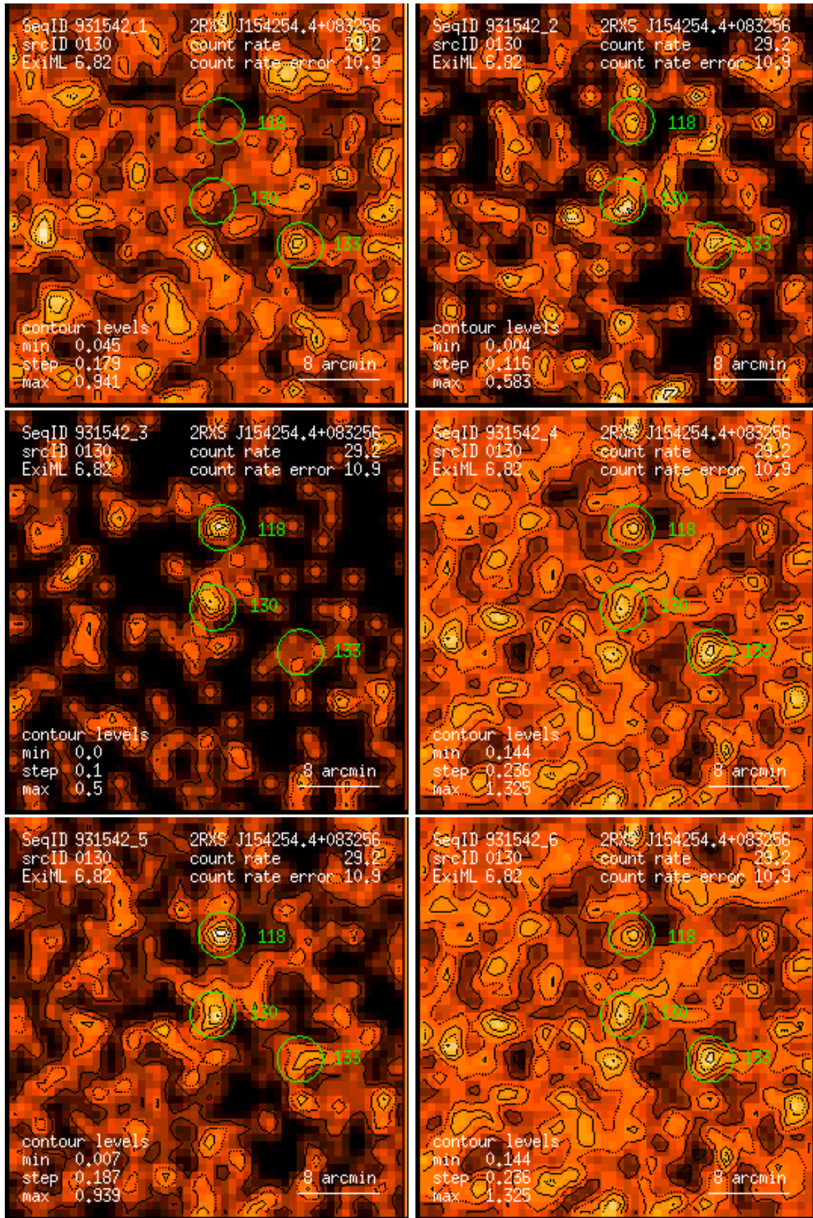
Figure 130: RASS 931542: detection 0130: band rate images, Gaussian filter: (1) PSPC channels 11 – 41, (2) 52 – 90, (3) 91 – 201, (4) 11 – 235, (5) 52 – 201, (6) 11 – 201. Broad band rates in counts/ks. Band rate contour levels in counts/ks/arcmin 2 .
