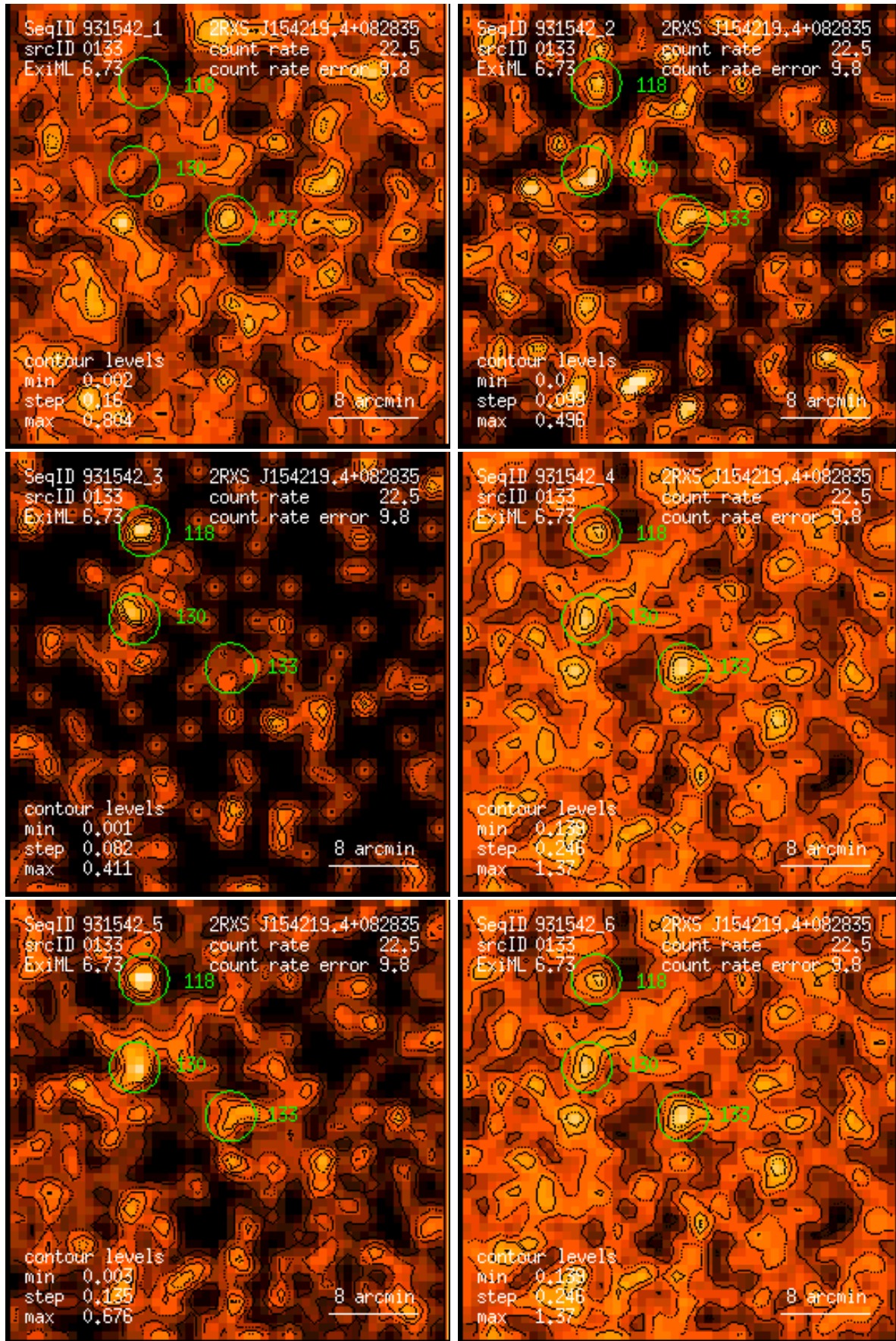
Figure 133: RASS 931542: detection 0133: band rate images, Gaussian filter: (1) PSPC channels 11 – 41, (2) 52 – 90, (3) 91 – 201, (4) 11 – 235, (5) 52 – 201, (6) 11 – 201. Broad band rates in counts/ks. Band rate contour levels in counts/ks/arcmin 2 .
