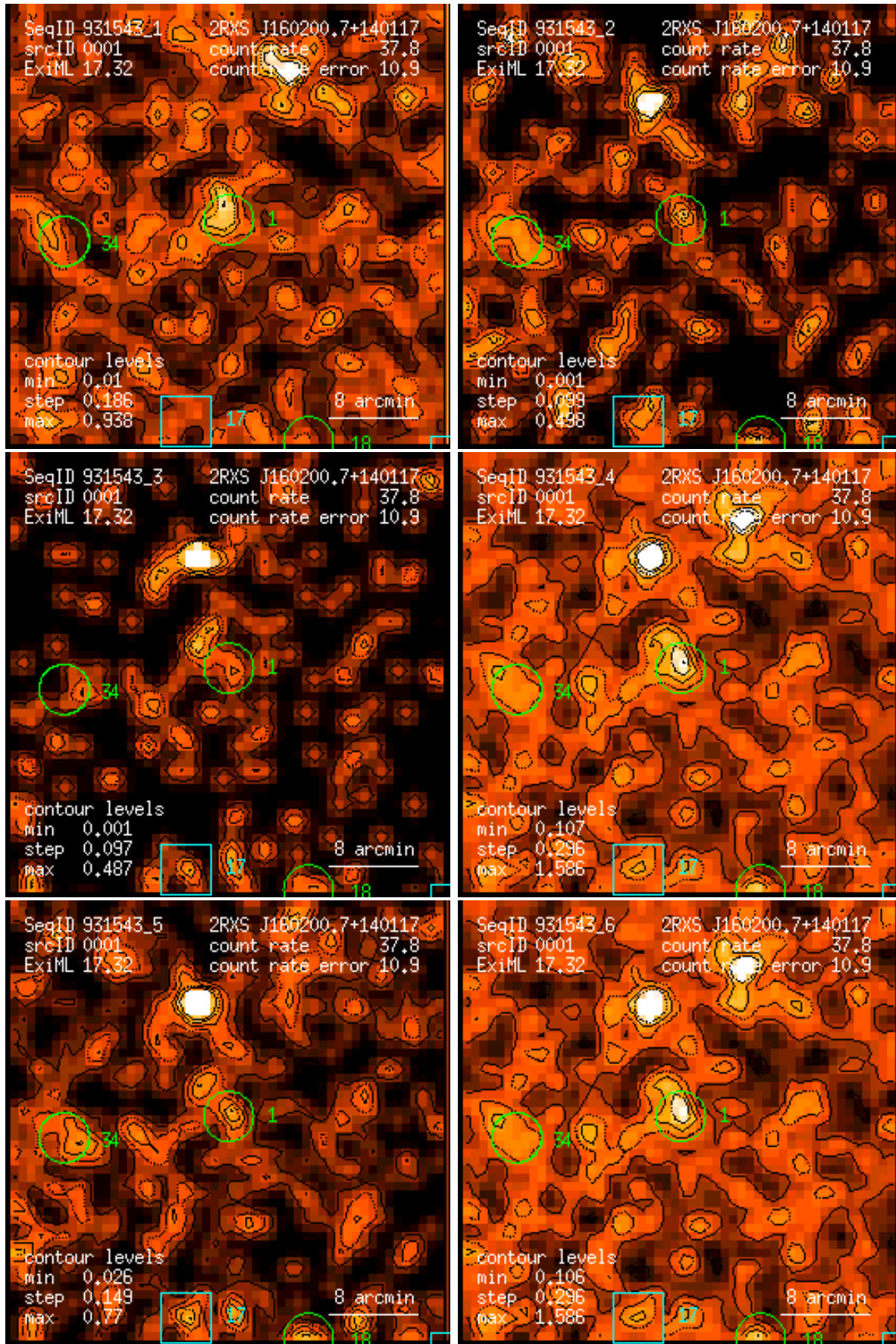
Figure 1: RASS 931543: detection 0001: band rate images, Gaussian filter: (1) PSPC channels 11 – 41, (2) 52 – 90, (3) 91 – 201, (4) 11 – 235, (5) 52 – 201, (6) 11 – 201. Broad band rates in counts/ks. Band rate contour levels in counts/ks/arcmin 2 .
