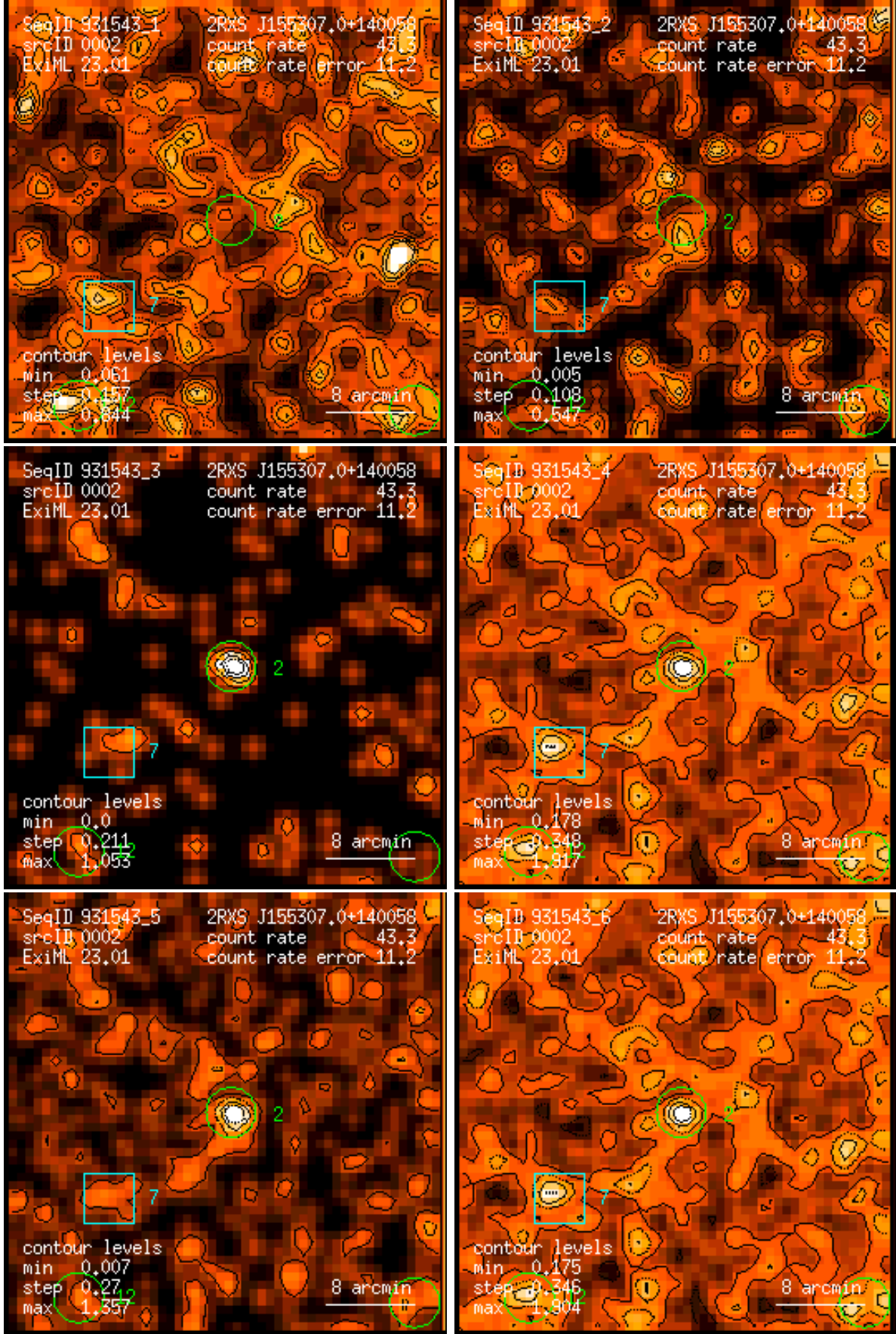
Figure 2: RASS 931543: detection 0002: band rate images, Gaussian filter: (1) PSPC channels 11 – 41, (2) 52 – 90, (3) 91 – 201, (4) 11 – 235, (5) 52 – 201, (6) 11 – 201. Broad band rates in counts/ks. Band rate contour levels in counts/ks/arcmin 2 .
