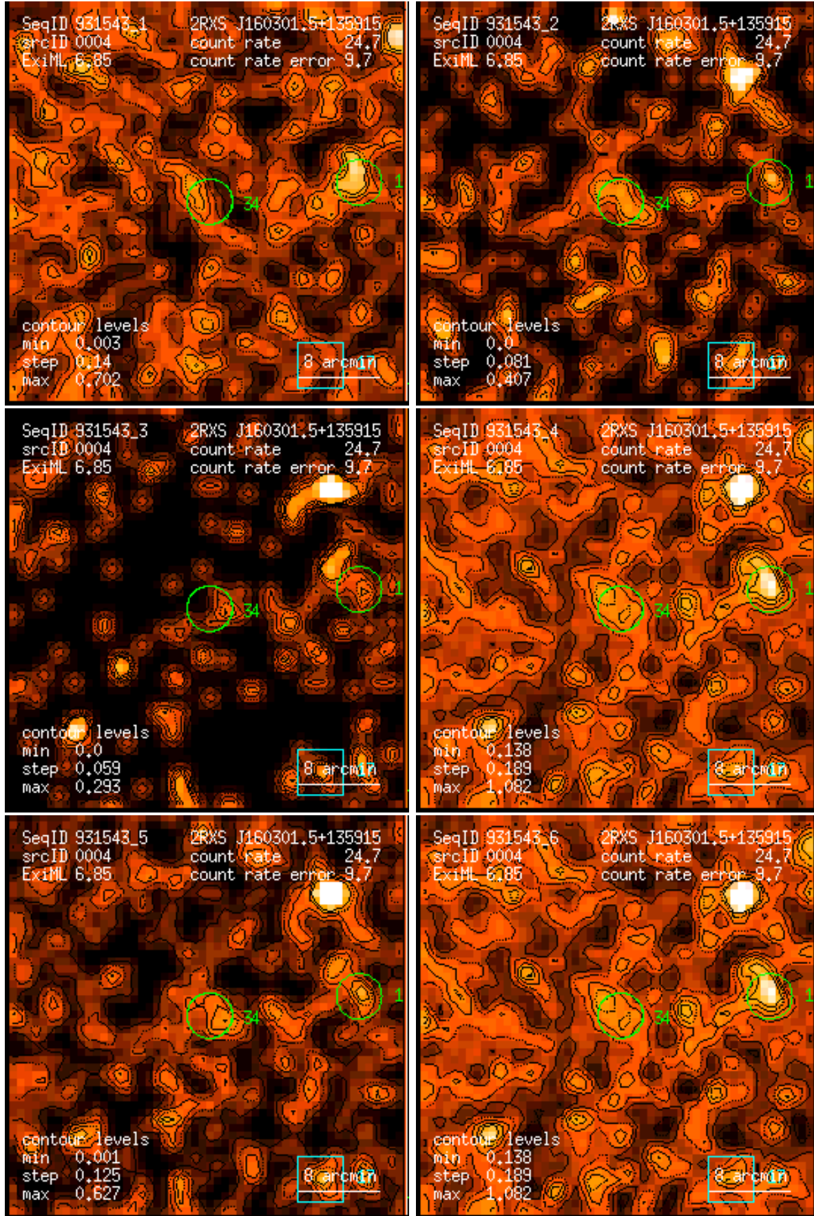
Figure 4: RASS 931543: detection 0004: band rate images, Gaussian filter: (1) PSPC channels 11 – 41, (2) 52 – 90, (3) 91 – 201, (4) 11 – 235, (5) 52 – 201, (6) 11 – 201. Broad band rates in counts/ks. Band rate contour levels in counts/ks/arcmin 2 .
