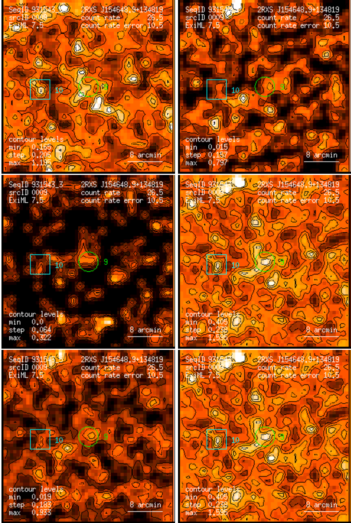
Figure 9: RASS 931543: detection 0009: band rate images, Gaussian filter: (1) PSPC channels 11 – 41, (2) 52 – 90, (3) 91 – 201, (4) 11 – 235, (5) 52 – 201, (6) 11 – 201. Broad band rates in counts/ks. Band rate contour levels in counts/ks/arcmin 2 .
