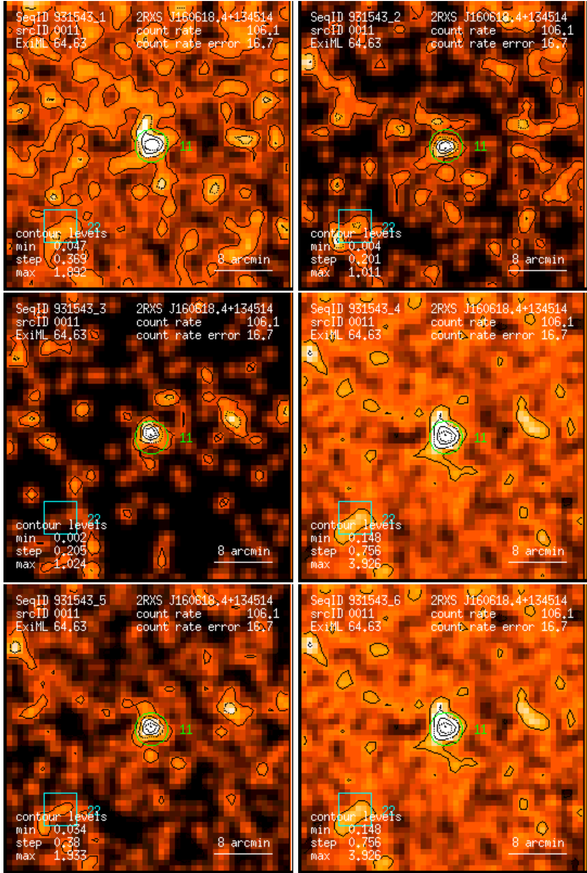
Figure 11: RASS 931543: detection 0011: band rate images, Gaussian filter: (1) PSPC channels 11 – 41, (2) 52 – 90, (3) 91 – 201, (4) 11 – 235, (5) 52 – 201, (6) 11 – 201. Broad band rates in counts/ks. Band rate contour levels in counts/ks/arcmin 2 .
