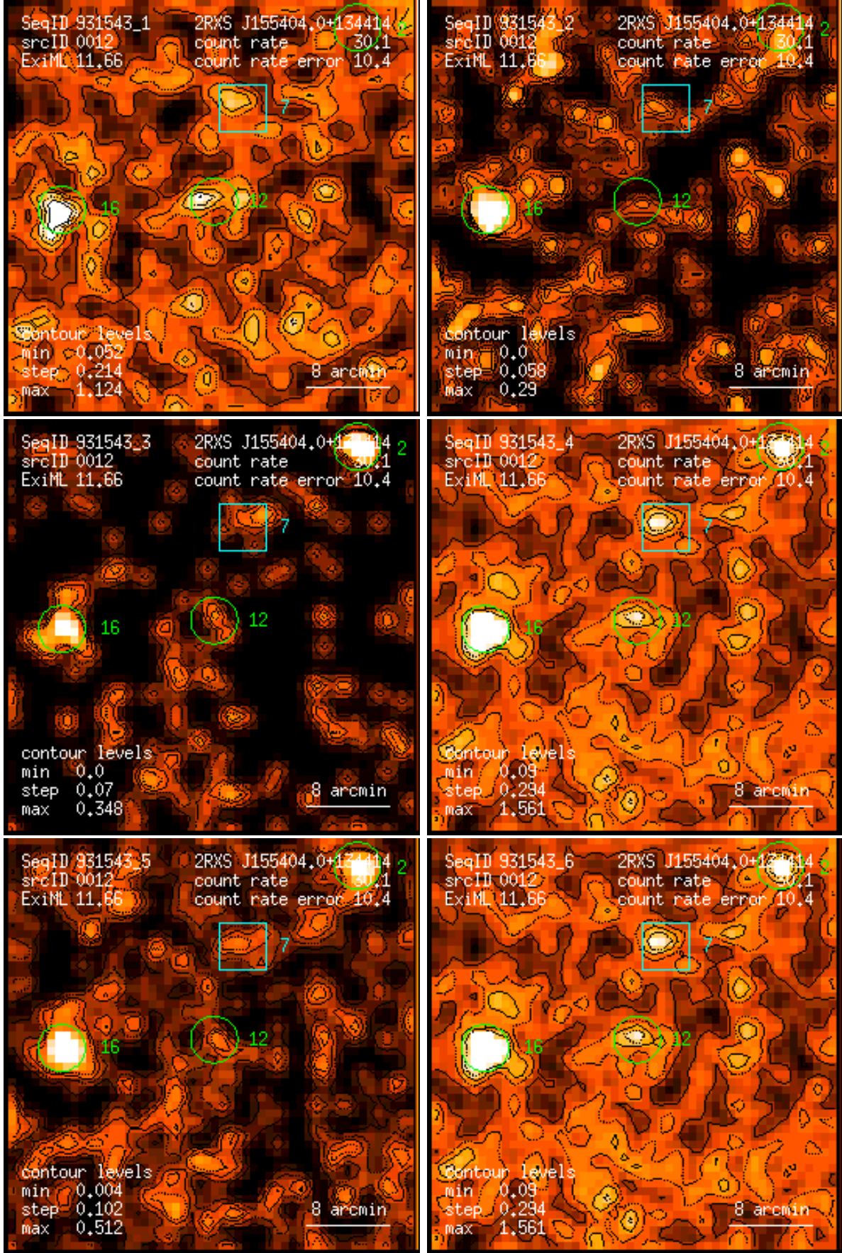
Figure 12: RASS 931543: detection 0012: band rate images, Gaussian filter: (1) PSPC channels 11 – 41, (2) 52 – 90, (3) 91 – 201, (4) 11 – 235, (5) 52 – 201, (6) 11 – 201. Broad band rates in counts/ks. Band rate contour levels in counts/ks/arcmin 2 .
