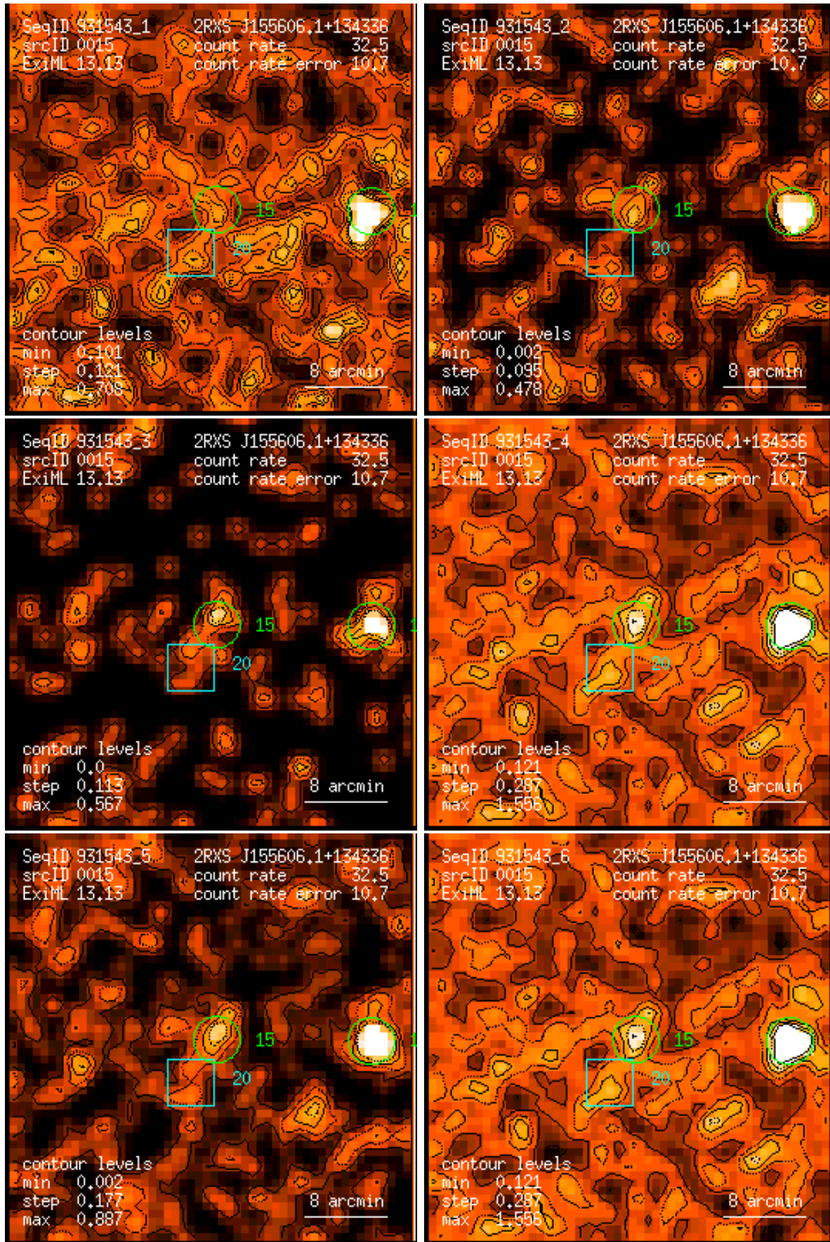
Figure 15: RASS 931543: detection 0015: band rate images, Gaussian filter: (1) PSPC channels 11 – 41, (2) 52 – 90, (3) 91 – 201, (4) 11 – 235, (5) 52 – 201, (6) 11 – 201. Broad band rates in counts/ks. Band rate contour levels in counts/ks/arcmin 2 .
