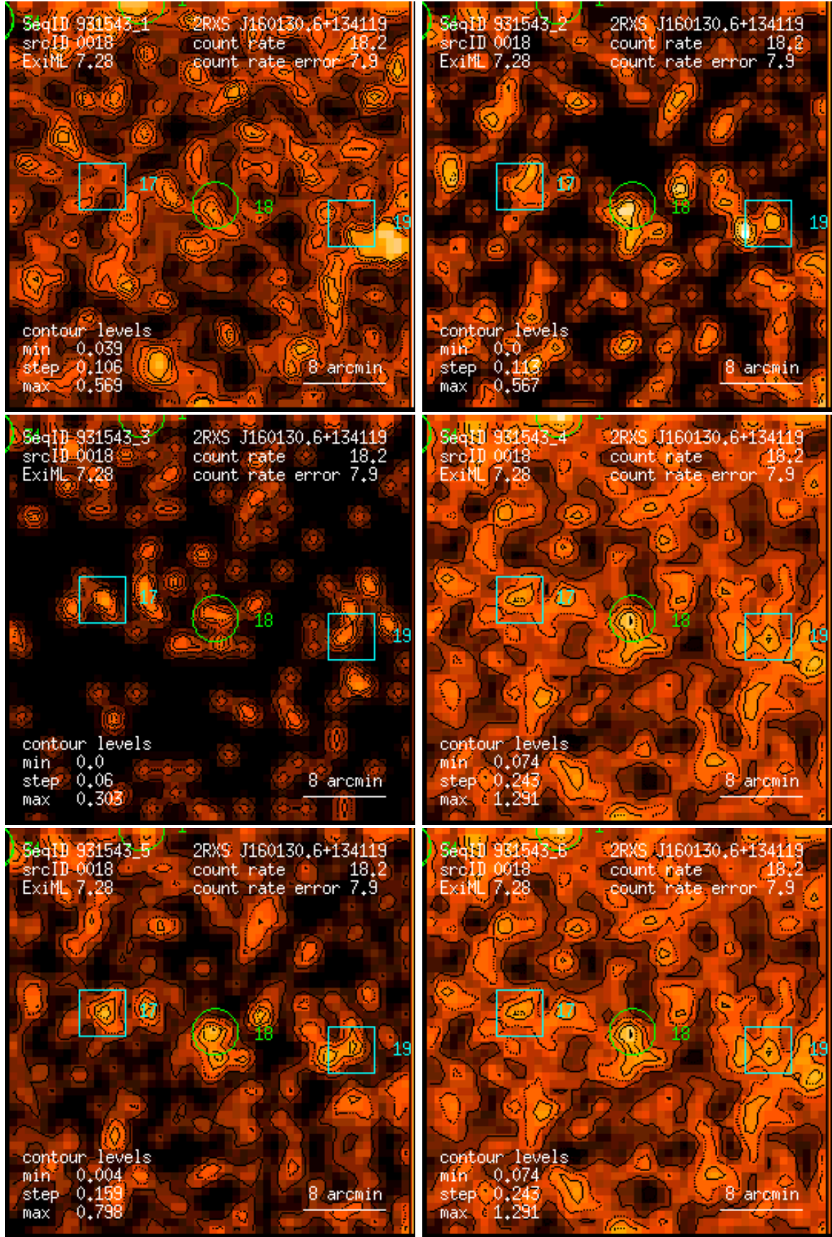
Figure 18: RASS 931543: detection 0018: band rate images, Gaussian filter: (1) PSPC channels 11 – 41, (2) 52 – 90, (3) 91 – 201, (4) 11 – 235, (5) 52 – 201, (6) 11 – 201. Broad band rates in counts/ks. Band rate contour levels in counts/ks/arcmin 2 .
