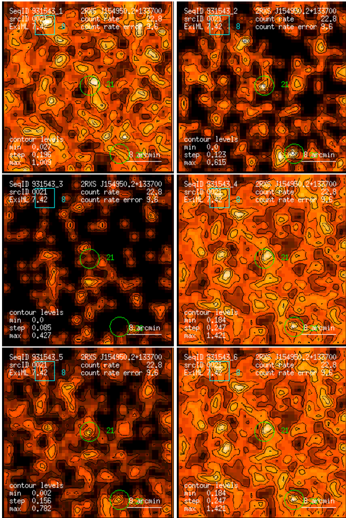
Figure 21: RASS 931543: detection 0021: band rate images, Gaussian filter: (1) PSPC channels 11 – 41, (2) 52 – 90, (3) 91 – 201, (4) 11 – 235, (5) 52 – 201, (6) 11 – 201. Broad band rates in counts/ks. Band rate contour levels in counts/ks/arcmin 2 .
