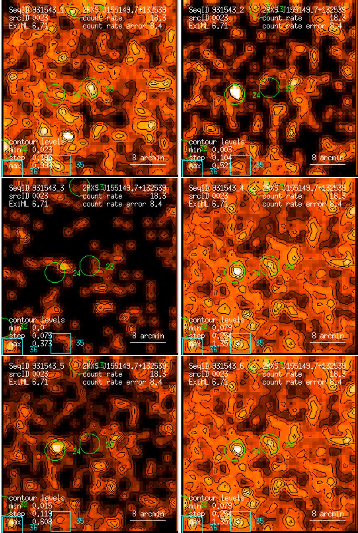
Figure 23: RASS 931543: detection 0023: band rate images, Gaussian filter: (1) PSPC channels 11 – 41, (2) 52 – 90, (3) 91 – 201, (4) 11 – 235, (5) 52 – 201, (6) 11 – 201. Broad band rates in counts/ks. Band rate contour levels in counts/ks/arcmin 2 .
